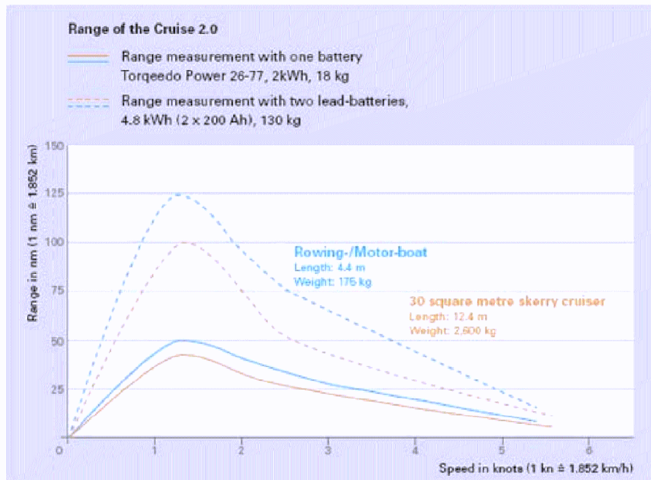
Figure 3. Range for torqeedo cruise, two different load cases.
