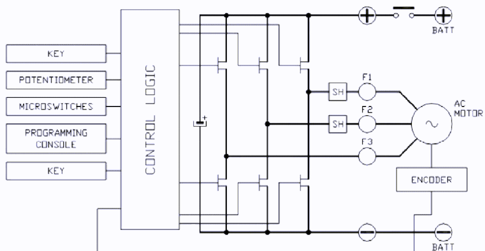
Figure 1. Example of connection of asynchronous motor with control system
