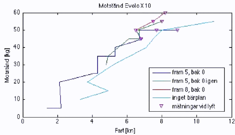
Figure 2. The same values as in Figure 1 but with markings on the measurement values that were recorded when Evolo had taken off.
