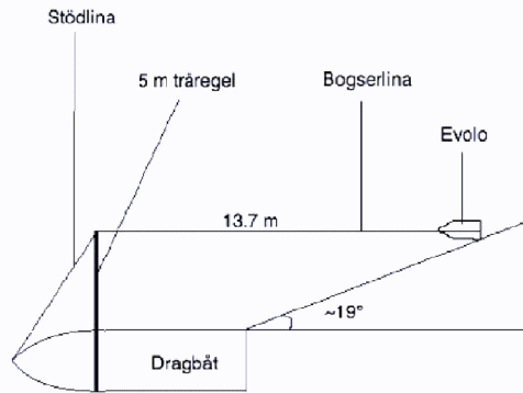
Figure 1. Anti-wake device.
