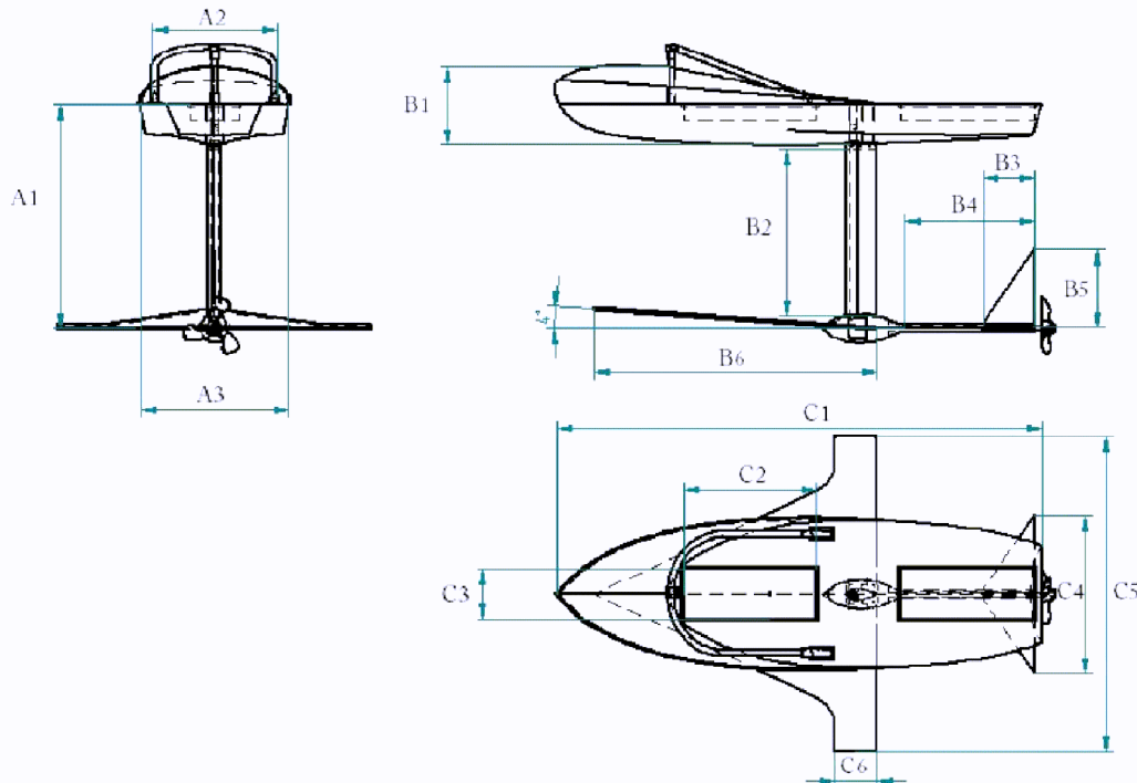
Figure. 8. General arrangement of Evolo
