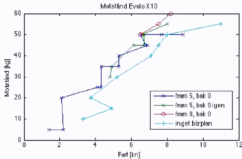
Figure 1. Measured resistances of Evolo with different hydrofoil angles.
