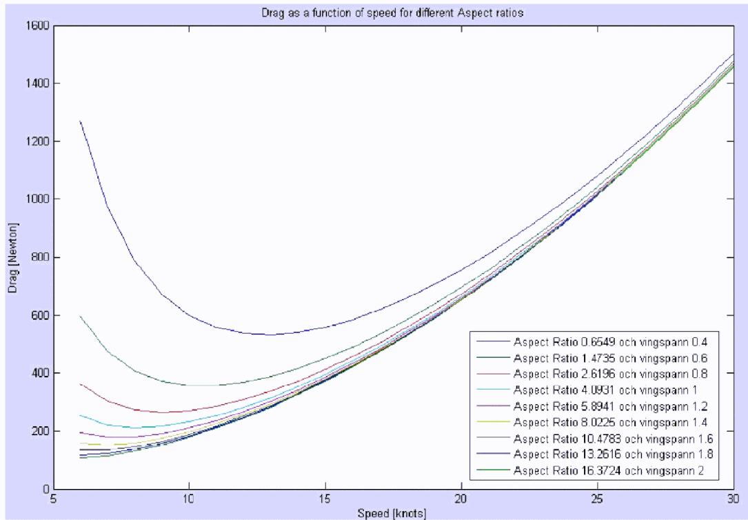
Figure 18. The resistance of the different hydrofoil plotted against the speed.
