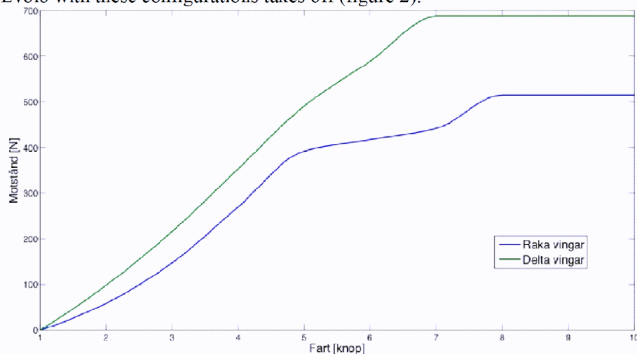
Figure 43. Resistance curve for Evolo.
