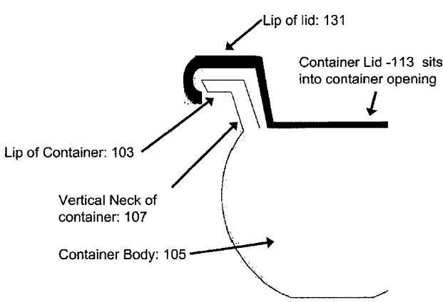
Side View - Lid & Lip of Container (Note: The lip and lid are enlarged to show hook)
