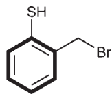
2-(bromomethyl)benzenethiol
