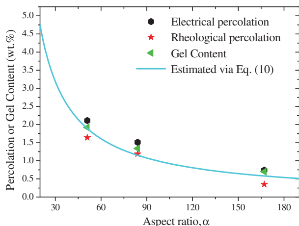
Fig. 11. Electrical percolation, rheological percolation, gel content values for MWCNT/PP composites and percolation values from estimation via Equation (10) as a function of aspect ratio.
