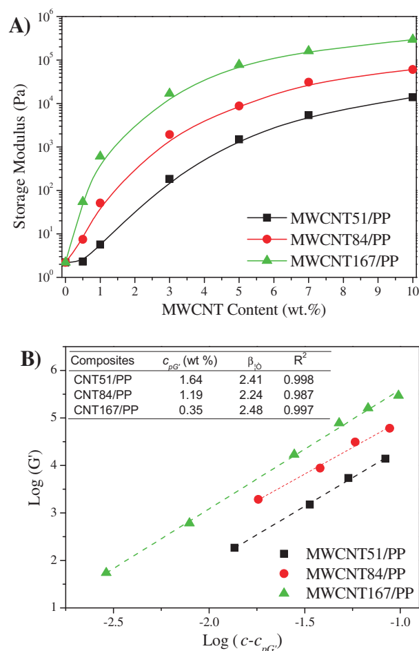
Fig. 6. (A) Storage modulus ( G' ) at an angular frequency of 0.5 rad/s for the MWCNT/PP composites as a function of MWCNT content. (B) A log–log plot of G' versus reduced mass fraction. Inset is the percolation parameters of respective MWCNT/PP composites.
