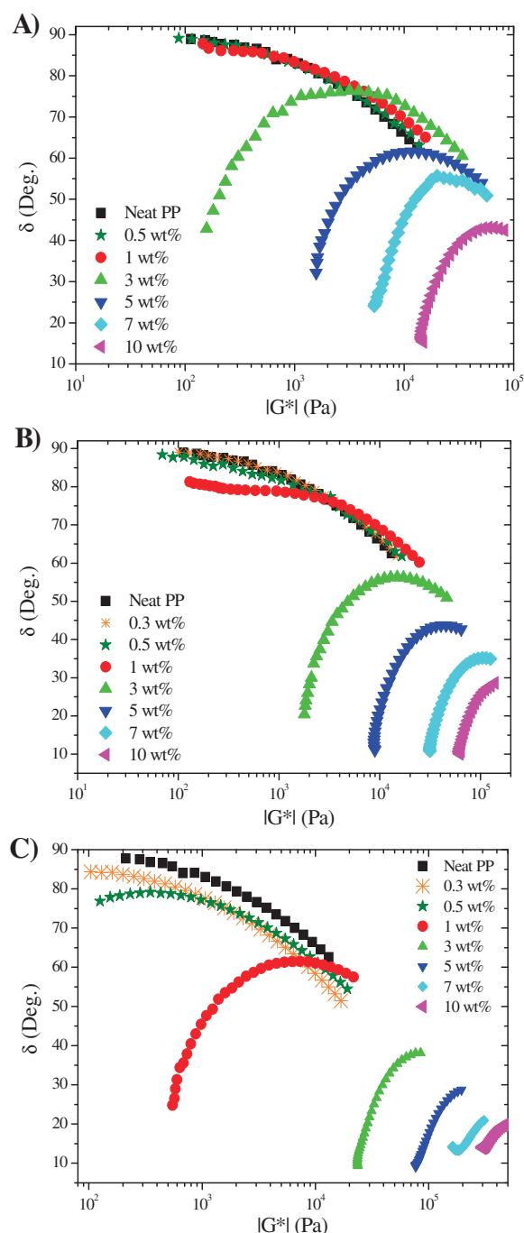
Fig. 5. Phase angle ( \delta ) as a function of dynamic complex modulus ( |G^*| ) for the PP composites containing various MWCNTs: (A) MWCNT51/PP, (B) MWCNT84/PP and (C) MWCNT167/PP.
