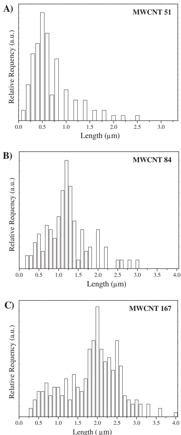
Fig. 1. Length distribution of different MWCNTs: (A) MWCNT51, (B) MWCNT84 and (C) MWCNT167.
