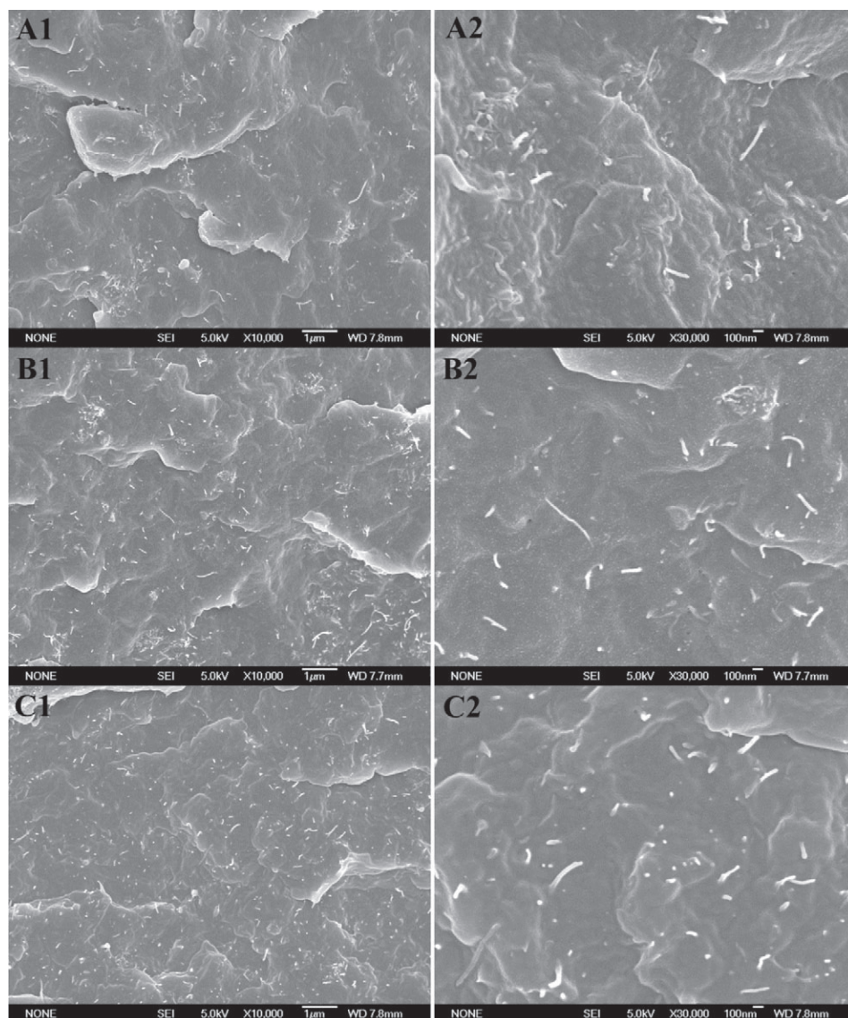
Fig. 3. FESEM images of different MWCNT/PP composites containing 3 wt% MWCNTs under different magnifications, (A) MWCNT51, (B) MWCNT84 and (C) MWCNT167.
