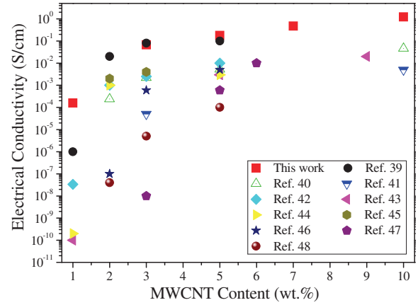
Fig. 10. Comparison of electrical conductivities with results in previous reports for MWCNT/PP composite systems [39–48].
