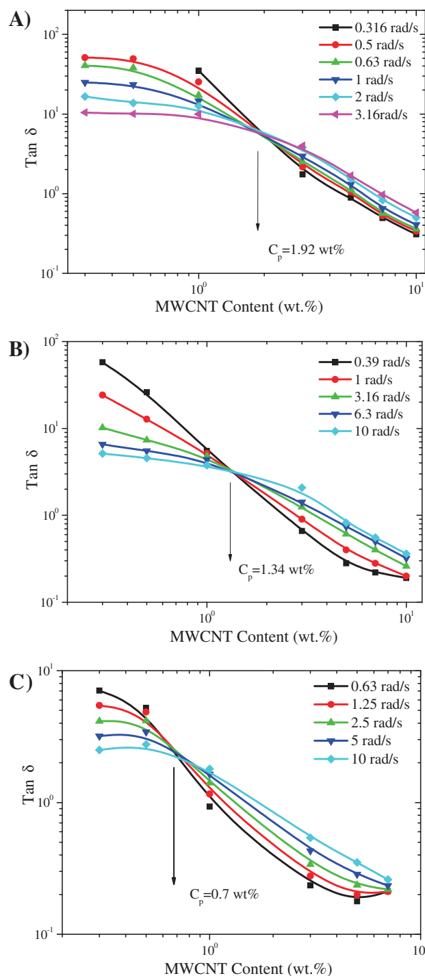
Fig. 7. Loss tangent ( \tan \delta ) as a function of MWCNT content for the PP composites containing various MWCNTs: (A) MWCNT51, (B) MWCNT84 and (C) MWCNT167. C_p is the MWCNT content at the gel point.
