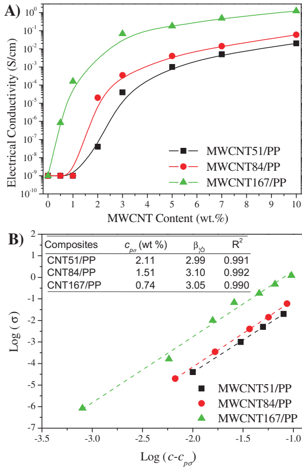
Fig. 9. (A) Electrical conductivity of the MWCNT/PP composites as a function of the MWCNT content. (B) A log–log plot of electrical conductivity versus reduced mass fraction. Inset is the percolation parameters for electrical properties of respective MWCNT/PP composites.
