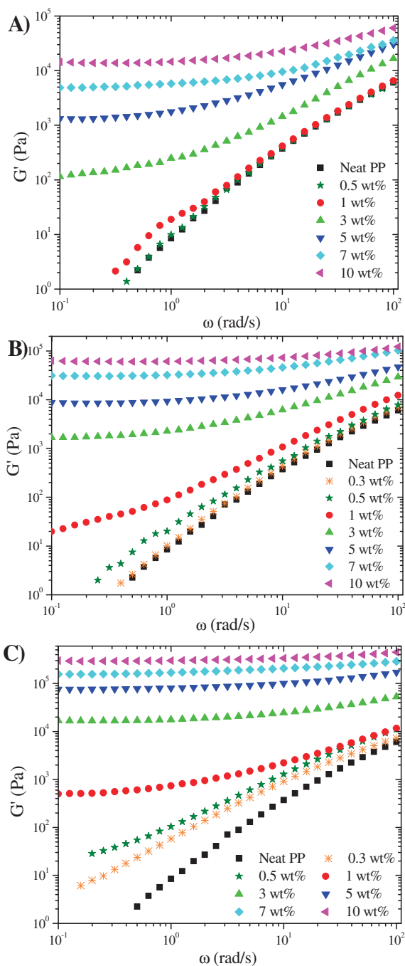
Fig. 4. Storage modulus ( G' ) as a function of angular frequency ( \omega ) for the composites containing various MWCNTs: (A) MWCNT51, (B) MWCNT84 and (C) MWCNT167.
