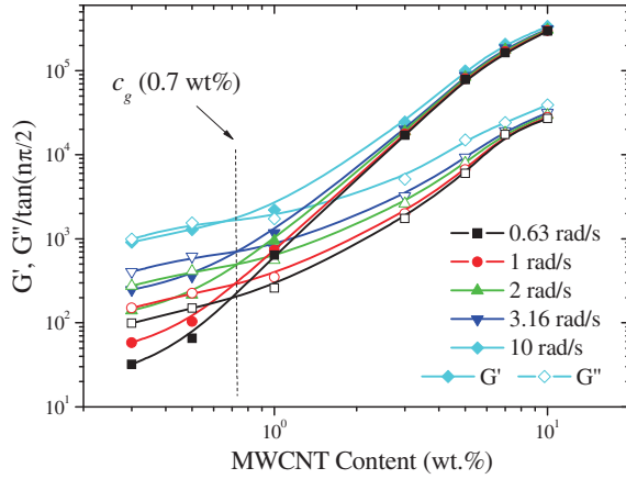
Fig. 8. Plots of G' and G''/\tan(\pi/2) versus MWCNT content for the MWCNT167/PP composites. The angular frequency was varied from 0.63 to 10 rad/s, n = 0.74 was used to calculate G''/\tan(\pi/2) . The gel point is indicated by the arrow.
