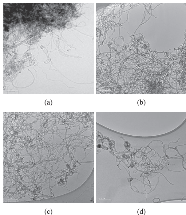
Figure 2. TEM images of CNT agglomerates dispersed according to Conditions A, B, C, and D described in Table 1 (scale bar = 0.2 \mu\text{m} ).
