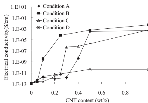
Figure 5. DC electrical conductivities of nanocomposites as a function of CNT content.
