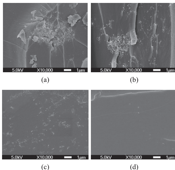
Figure 3. SEM images of 0.1 wt % CNT-epoxy nanocomposites dispersed according to Conditions A, B, C, and D described in Table 1 (scale bar = 1 \mu\text{m} ).
