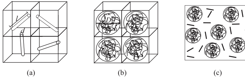
Figure 7. Cartoons of CNT-reinforced polymer nanocomposites containing a) perfectly dispersed cylindrical CNTs, b) CNTs all in the form of agglomerates, and c) a mixture of individual CNTs and agglomerates.
