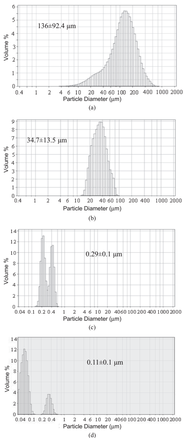
Figure 1. Size distributions of CNT agglomerates produced according to a) Condition A, b) Condition B, c) Condition C, and d) Condition D, before being embedded in an epoxy resin.
