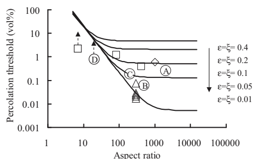
Figure 9. Effect of aspect ratio on the percolation threshold of CNT-reinforced polymer nanocomposites with varying dispersion states. Experimental data: Conditions A, B, C and D in the present study ○; □ [6]; □ [7] and □ [8].
