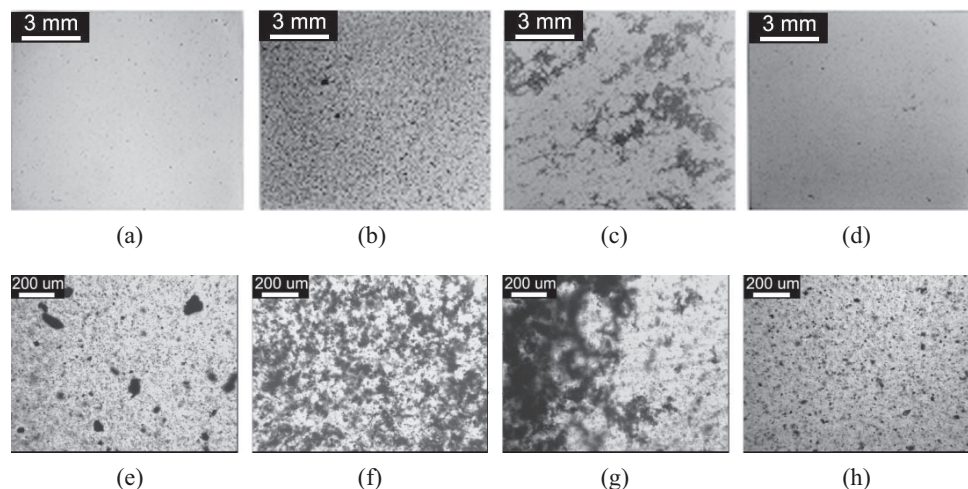
Figure 4. Transmission mode optical microscopy images of 0.05 wt % CNT-epoxy nanocomposites for Conditions A through D at different magnifications.
