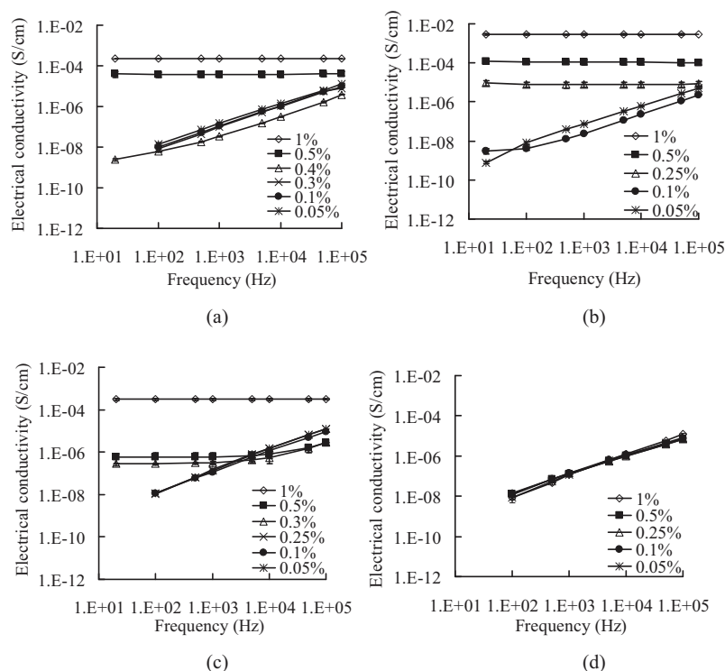
Figure 6. Frequency dependence of the AC conductivity of nanocomposites produced by a) Condition A, b) Condition B, c) Condition C, and d) Condition D.
