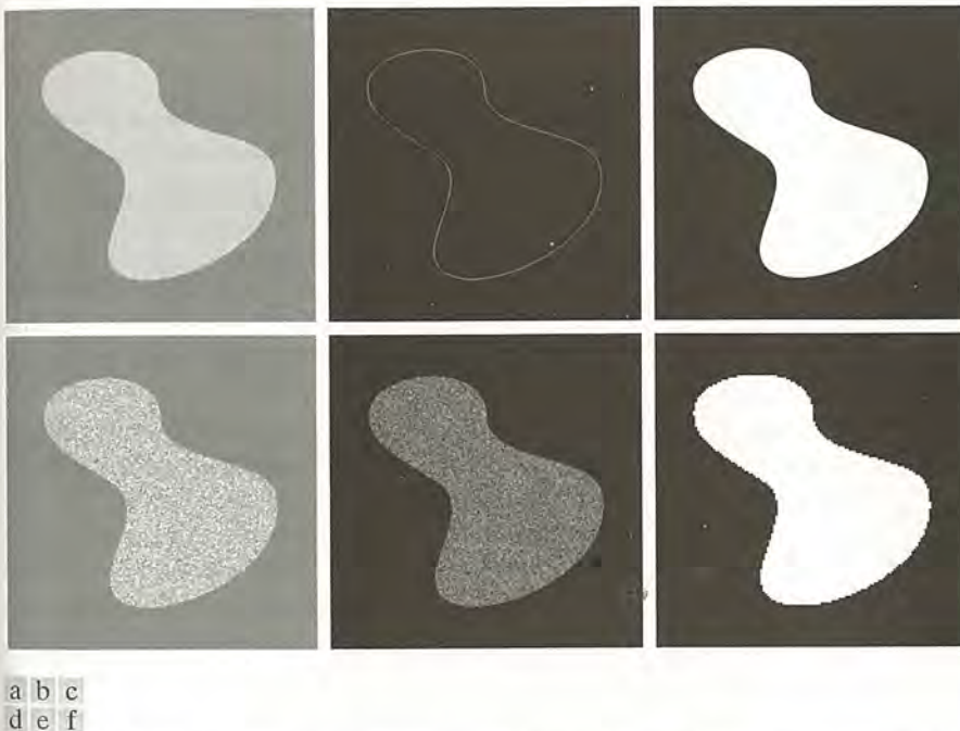
FIGURE 10.1 (a) Image containing a region of constant intensity. (b) Image showing the boundary of the inner region, obtained from intensity discontinuities. (c) Result of segmenting the image into two regions. (d) Image containing a textured region. (e) Result of edge computations. Note the large number of small edges that are connected to the original boundary, making it difficult to find a unique boundary using only edge information. (f) Result of segmentation based on region properties.
