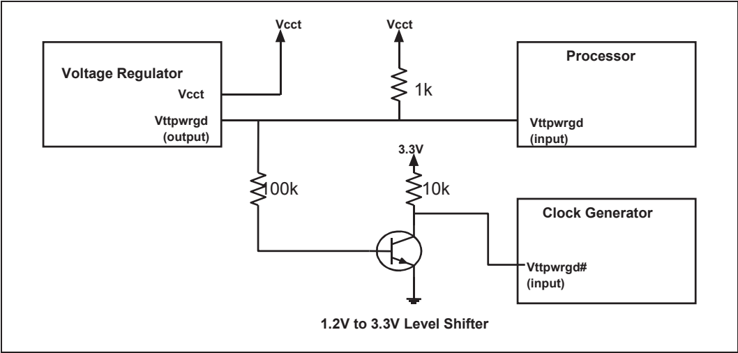
Figure 3. VTPWRGD System-Level Connections
