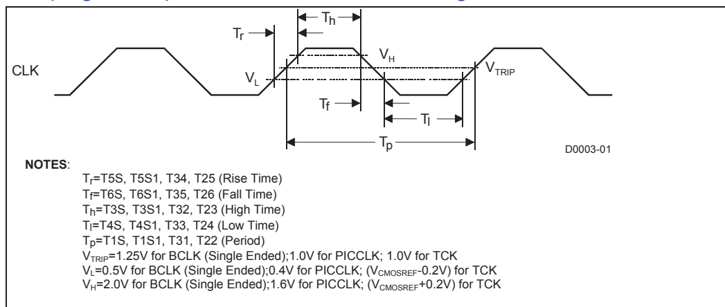
Figure 9. BCLK (Single Ended)/PICCLK/TCK Generic Clock Timing Waveform
