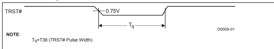
Figure 19. Test Reset Timings
