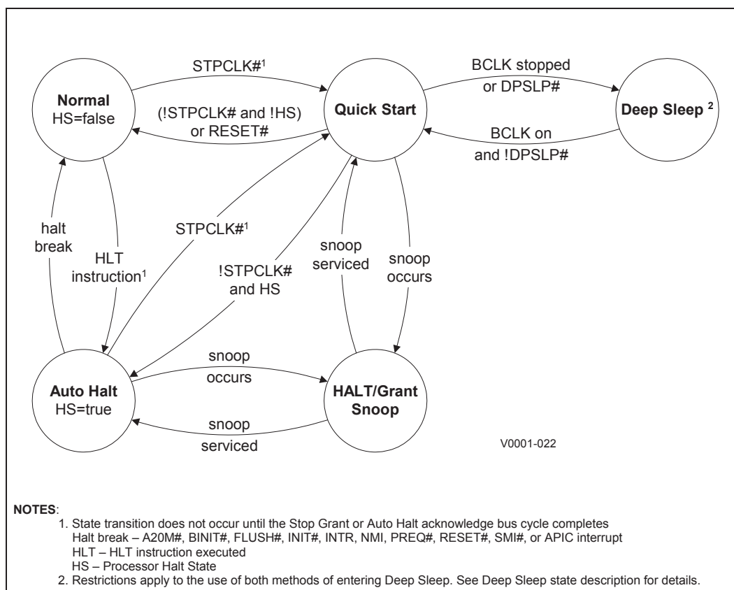
Figure 1. Clock Control States
