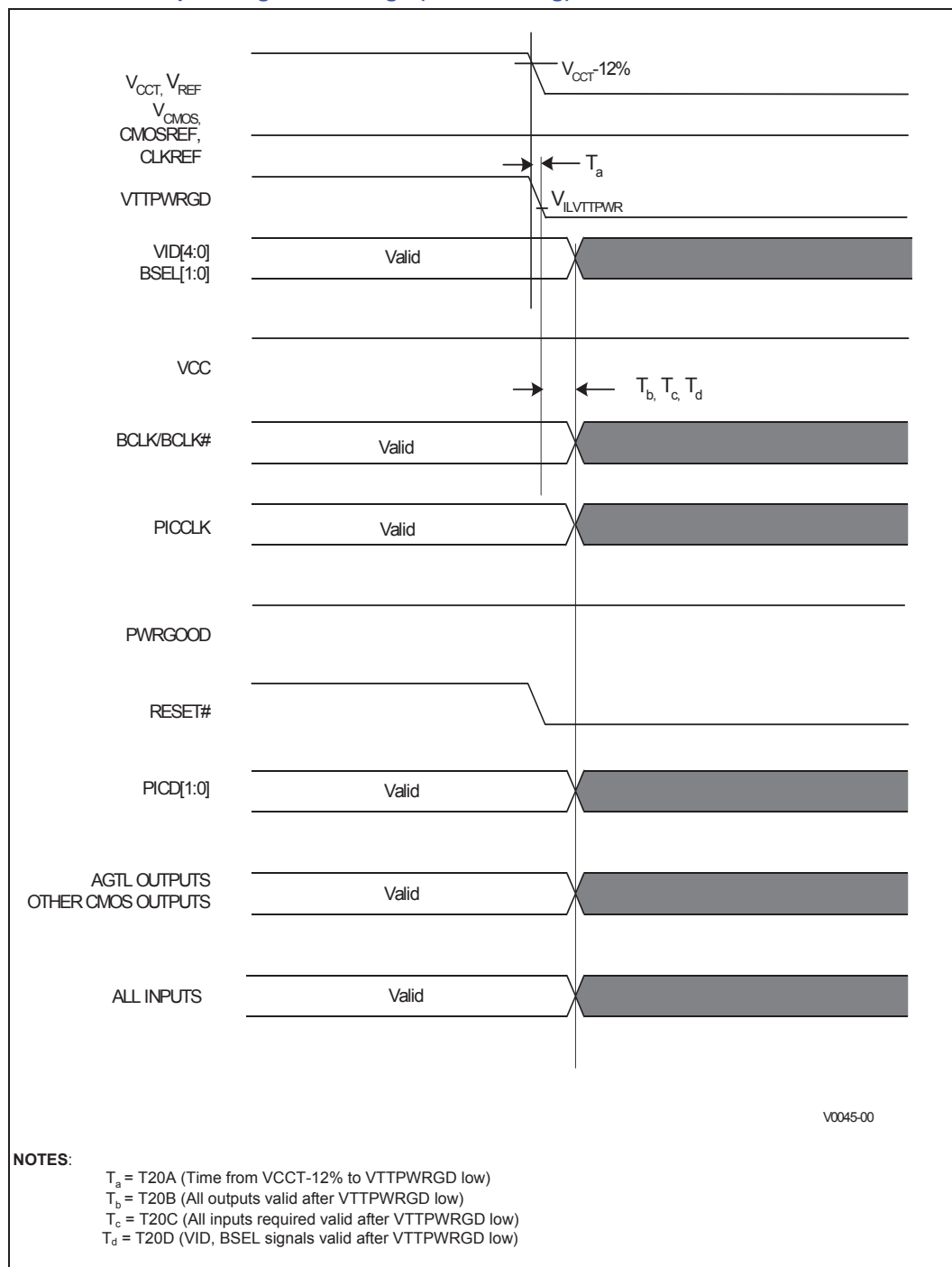
Figure 17. Power Down Sequencing and Timings ( V_{CCT} Leading)
