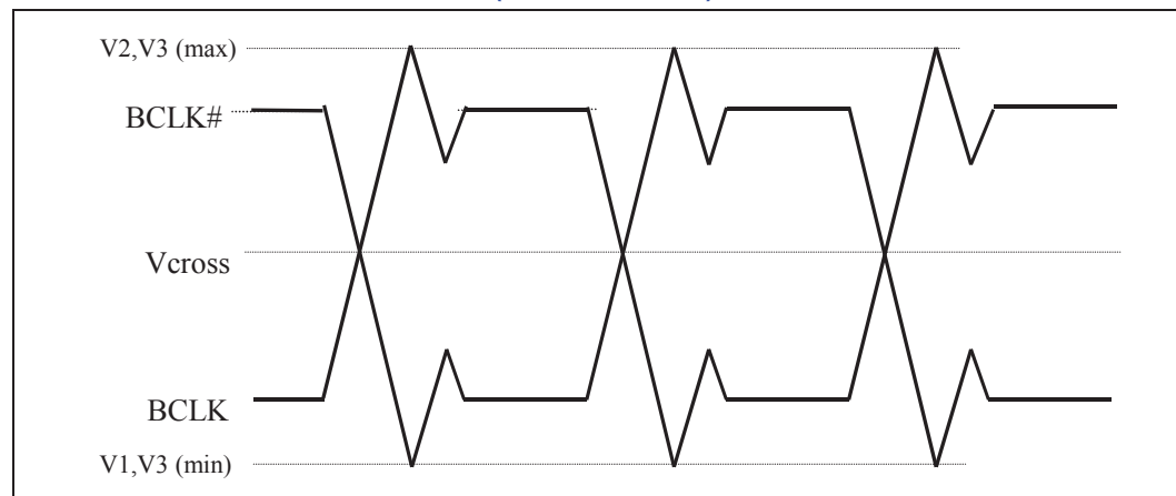
Figure 10. Differential BCLK/BCLK# Waveform (Common Mode)
