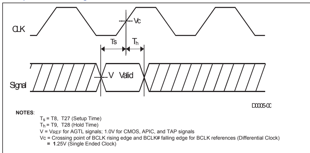
Figure 13. Setup and Hold Timings
