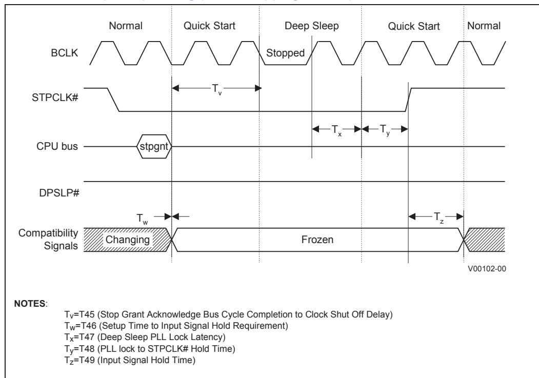
Figure 20. Quick Start/Deep Sleep Timing (BCLK Stopping Method)
