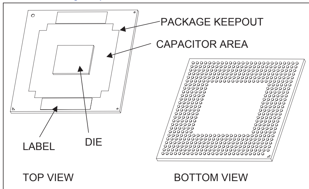
Figure 28. Micro-FCBGA Package – Top and Bottom Isometric Views
