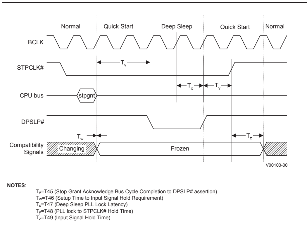
Figure 21. Quick Start/Deep Sleep Timing (DPSLP# Assertion Method)
