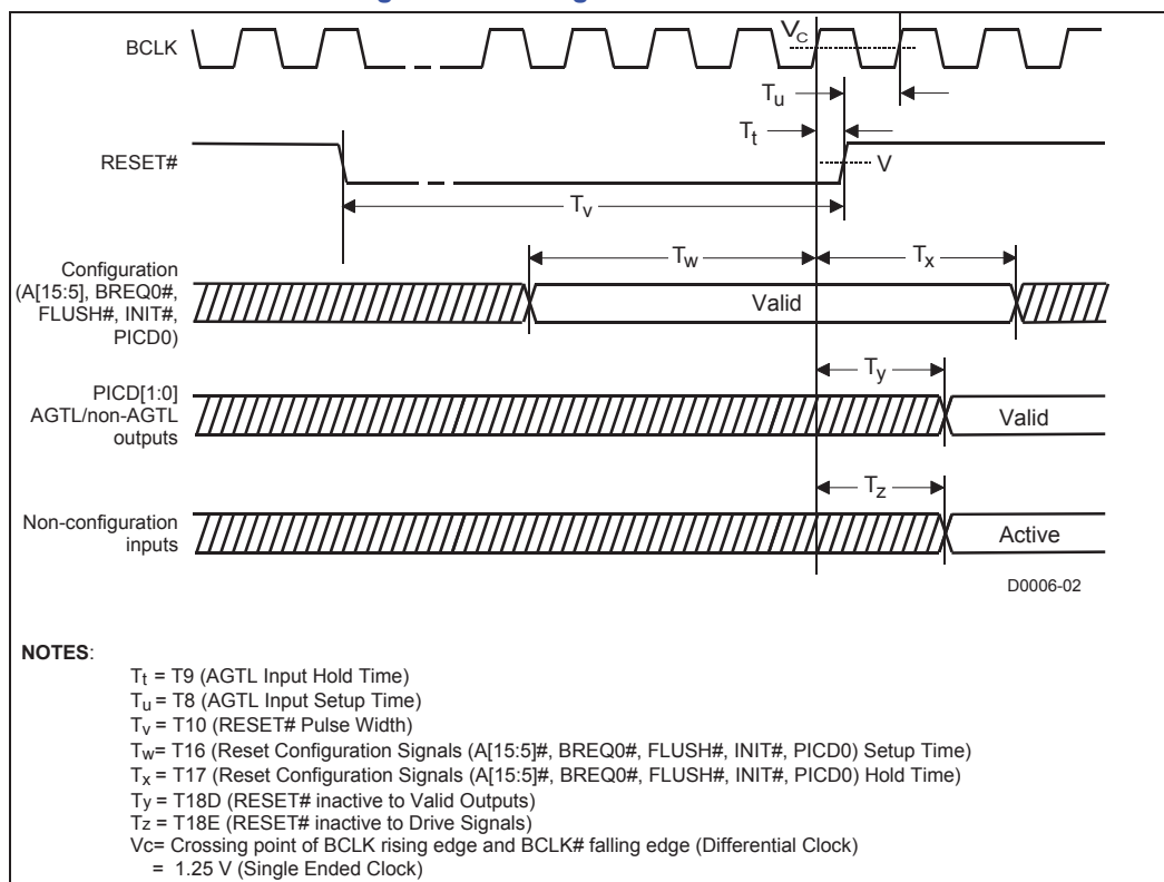
Figure 14. Cold/Warm Reset and Configuration Timings
