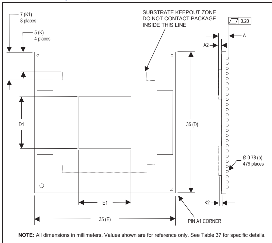
Figure 29. Micro-FCBGA Package – Top and Side Views
