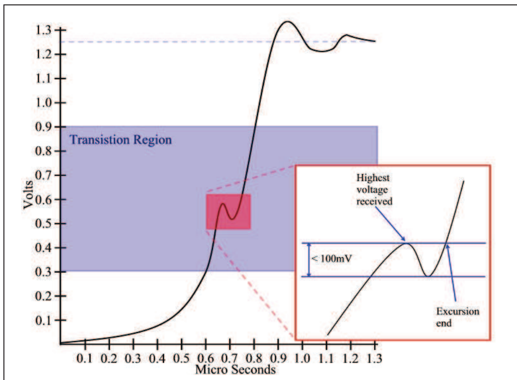
Figure 4. Noise Estimation
