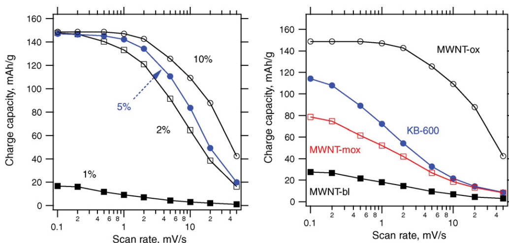
Fig. 10. Integral voltammetric charge capacity as a function of scan rate. (Left chart): \text{LiFePO}_4 in a composite with functionalized nanotubes, MWNT-ox. The concentration of MWNT-ox in the composite varied between 1 and 10 wt% (as in Fig. 9). (Right chart): \text{LiFePO}_4 in a composite with the following carbonaceous materials: oxidized nanotubes (MWNT-ox; 2.54 \times 10^{-4} \text{ mol g}^{-1} acidic groups), medium-functionalized nanotubes (MWNT-mox; 1.14 \times 10^{-4} \text{ mol g}^{-1} acidic groups), non-functionalized nanotubes (MWNT-bl) and carbon black KB-600. The concentration was 10 wt% in all composites shown in the left chart.
