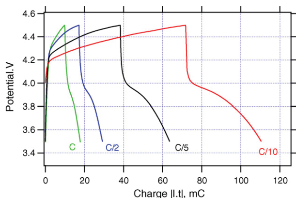
Fig. 11. Galvanostatic chronopotentiometry of \text{LiMnPO}_4 in a composite with 10 wt% of functionalized nanotubes, MWNT-ox (film mass 0.62 \text{ mg cm}^{-2} ). Discharge/charge cycles are shown for varying charge rates from C/10 to C.
