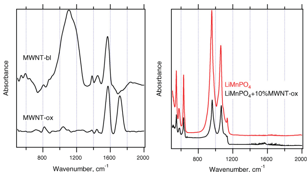
Fig. 4. Left panel: FTIR spectra in KBr pellets of non-functionalized and functionalized nanotubes, MWNT-bl and MWNT-ox, respectively. Right panel: ATR-FTIR spectra of powder of pure LiMnPO 4 and LiMnPO 4 in a composite with 10 wt% of functionalized nanotubes MWNT-ox. Spectra are offset for clarity.
