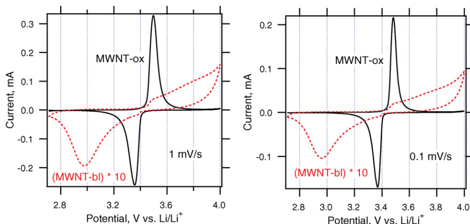
Fig. 8. Cyclic voltammograms of LiFePO 4 thin film electrodes. Black full curve: LiFePO 4 in a composite with 10 wt% of functionalized nanotubes, MWNT-ox (film mass 0.33 mg cm -2 ). Red dashed curve: LiFePO 4 in a composite with 10 wt% of non-functionalized MWNT-bl (film mass 0.38 mg cm -2 ); this curve is zoomed by a factor of 10 in the current scale. Scan rate 1 or 0.1 mV s -1 for the left or right charts, respectively.
