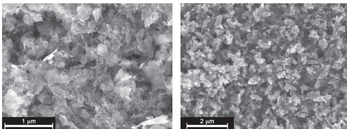
Fig. 3. Scanning electron microscopy images of thin film electrodes from phosphate olivines in a composite with 10 wt% of functionalized nanotubes, MWNT-ox. (Left) Composite with LiMnPO 4 , scale bar 1 μm. (Right) Composite with LiFePO 4 , scale bar 2 μm.
