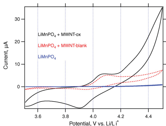
Fig. 7. Cyclic voltammograms of LiMnPO 4 thin film electrodes in a composite with 10 wt% of MWNT-ox (film mass 0.83 mg cm -2 ). Red dashed curve: LiMnPO 4 in a composite with 10 wt% of MWNT-bl, film mass 0.87 mg cm -2 ; the same film like in Fig. 6). Blue curve: pure LiMnPO 4 (film mass 1.05 mg cm -2 ) Scan rate 0.2 mV s -1 .
