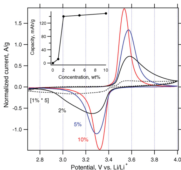
Fig. 9. Cyclic voltammograms of LiFePO 4 in a composite with functionalized nanotubes, MWNT-ox. The concentration of MWNT-ox in the composite varied between 1 and 10 wt%. Currents are normalized to the actual mass of LiFePO 4 in the thin-film electrode, and for the voltammogram of 1 wt% composite, the current was zoomed by a factor of 5. Scan rate 0.5 mV s -1 . Inset shows the integral voltammetric charge capacity as a function of the concentration of MWNT-ox in the composite.
