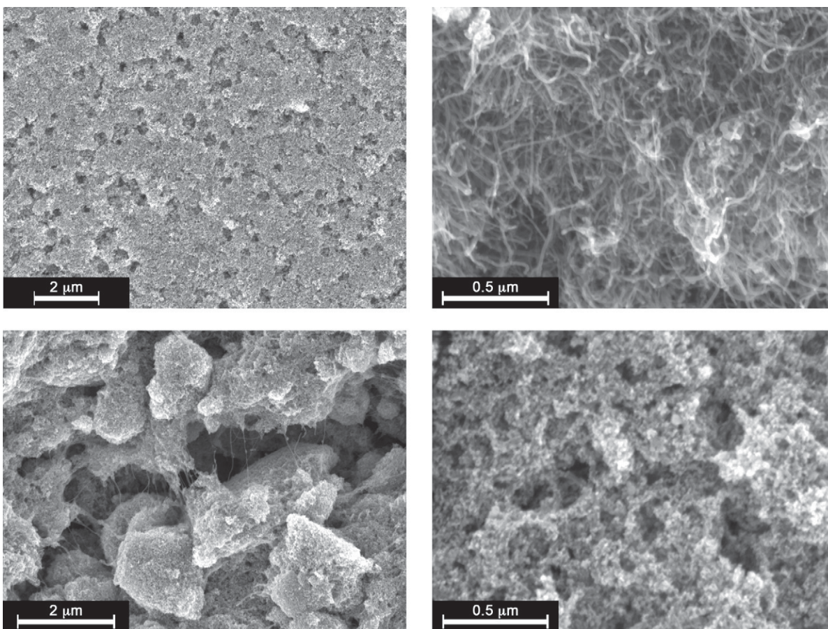
Fig. 2. Scanning electron microscopy images of thin film electrodes from P90 titanium dioxide. (Top left) Pure P90, scale bar 2 μm. (Top right) pure functionalized nanotubes MWNT-ox, scale bar 0.5 μm. (Bottom left) P90 in a composite with 10 wt% of non-functionalized nanotubes MWNT-bl, scale bar 2 μm. (Bottom right) P90 in a composite with 10 wt% of functionalized MWNT-ox, scale bar 0.5 μm.
