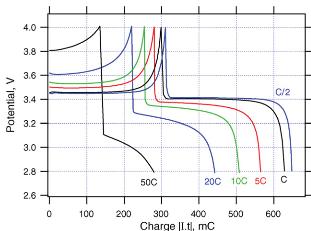
Fig. 12. Galvanostatic chronopotentiometry of \text{LiFePO}_4 in a composite with 10 wt% of functionalized nanotubes, MWNT-ox (film mass 0.68 \text{ mg cm}^{-2} ). Discharge/charge cycles are shown for varying charge rates from C/2 to 50C.
