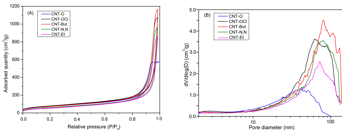
Figure 1. (A) Isotherms and (B) BJH distribution (adsorption branch) curves for CNT-O, CNT-OCI, and CNT-A samples.
