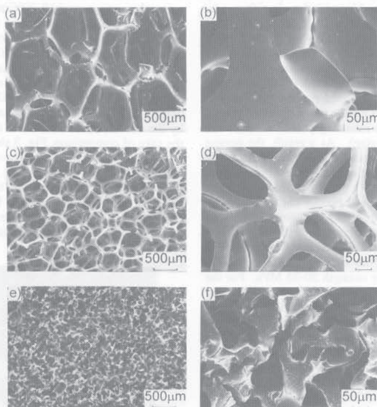
Fig. 3. SEM photographs of phenolic based porous carbons (a) and (b) 45 ppi, (c) and (d) 100 ppi, (e) and (f) 500 ppi.
