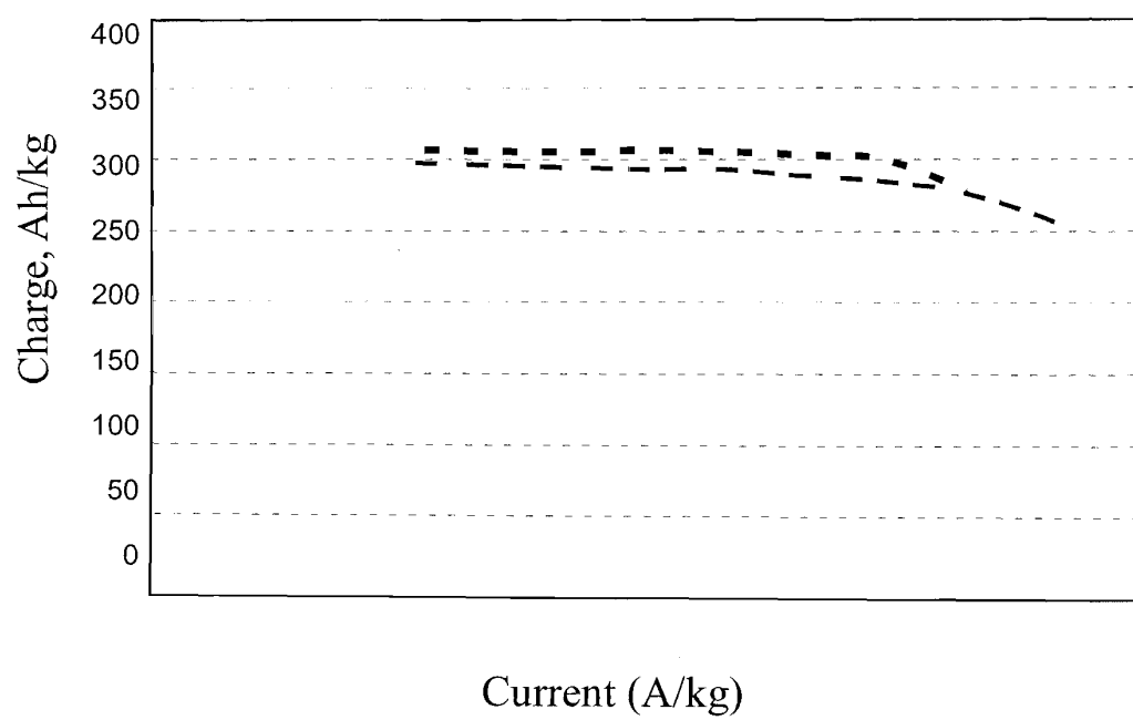
Anode: Capacity v. Current
