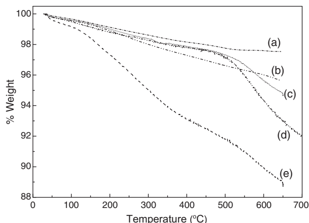
Fig. 6 – TGA curves of the MWCNT samples: (a) MWCNT- \text{NH}_4\text{OH}/\text{H}_2\text{O}_2 , (b) MWCNT- \text{H}_2\text{SO}_4/\text{H}_2\text{O}_2 , (c) MWCNT-HCl, (d) as-received and (e) MWCNT- \text{HNO}_3 .
