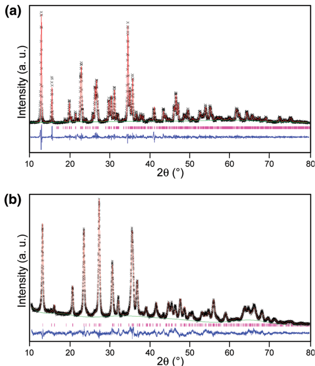
Figure 7. (a) LeBail XRD refinement of \text{Na}_{1.5}\text{FePO}_4\text{F} in P2/c , wRp = 9.07\% : lattice parameters a = 13.929(6) Å, b = 5.200(9) Å, c = 11.514(7) Å; \beta = 91.22^\circ . (b) Rietveld refinement of \text{Li}_{1.25}\text{Na}_{0.75}\text{FePO}_4\text{F} , synthesized from \text{NaFePO}_4\text{F} reduced with excess Li in Pbcn , wRp = 7.69\% : lattice parameters a = 5.0327(3) Å, b = 13.8590(7) Å, c = 11.2081(5) Å. For each, the fit is shown in red, the calculated reflections are shown in magenta, the background fit is shown in green and the difference map is shown in blue.
