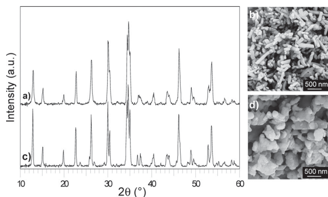
Figure 2. Powder diffraction patterns and corresponding SEM micrographs of \text{Na}_2\text{FePO}_4\text{F} (a) and (b) prepared hydrothermally (lattice parameters a = 5.231 Å, b = 13.887 Å, c = 11.806 Å); (c and d) prepared by a solid-state route (lattice parameters: a = 5.218 Å, b = 13.854 Å, c = 11.779 Å).
