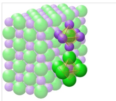
Crystal structure of sodium chloride (NaCl) with sodium cations ( \text{Na}^+ ) in purple and chloride anions ( \text{Cl}^- ) in green. The yellow stipples represent the electrostatic force between the ions of opposite charge.
