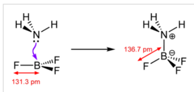
Adduct of ammonia and boron trifluoride
