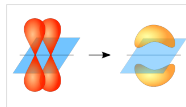
Two p-orbitals forming a pi-bond.
