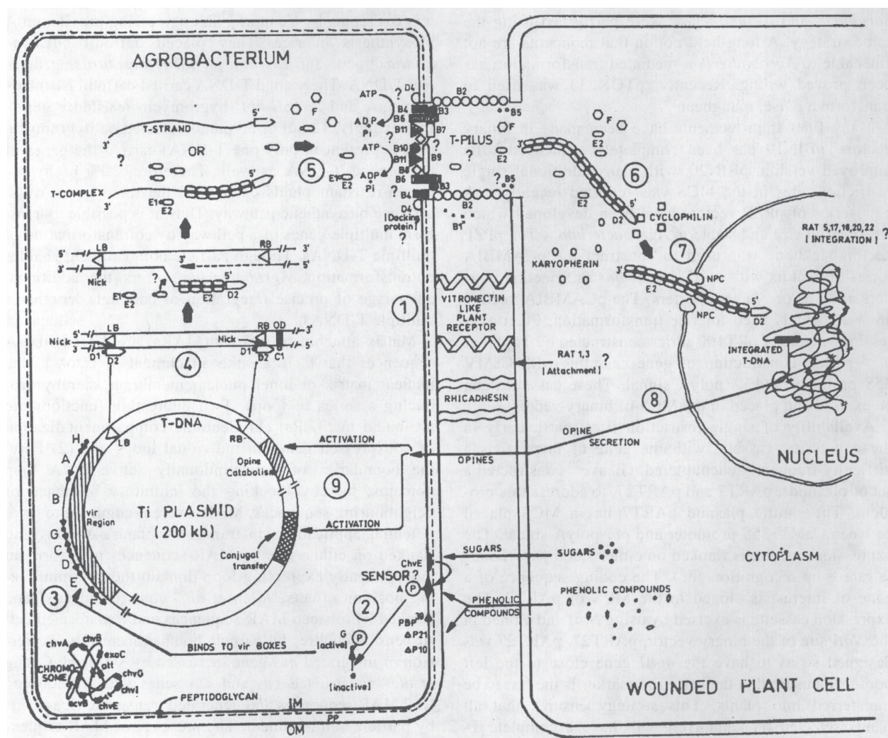
Figure 1. A schematic diagram depicting the cascade of events leading to T-DNA transfer from Agrobacterium to the plant genome. Steps 1 through 9 indicate sequential processes that occur during infection of a plant cell with Agrobacterium . Step 1, binding of Agrobacterium to the host cell surface receptors; step 2, direct or indirect mode of recognition of plant signal molecules by the bacterial Vir A/VirG two-component sensor-transducer system; step 3, induction of bacterial vir genes situated on the Ti plasmid; step 4, generation of the T-strand; step 5, formation of the T-complex and its transport into the host plant cell through the T-pilus; step 6, recognition and interaction of T-complex with host cell cytoplasmic proteins; step 7, nuclear transport of T-complex; step 8, T-DNA integration and opine secretion; and step 9, activation of bacterial opine catabolism genes and Ti plasmid conjugal transfer genes. acvB , att , chvA , chvB , chvC , chvE , chvG , chvI and exoC are the chromosome-encoded virulence genes. '?' Indicates that precise steps are yet to be established. P10, P21 and PBP are chromosome-encoded putative phenol-binding proteins. OM, outer membrane; PP, periplasm; IM, inner membrane. Broken lines denote peptidoglycan cell wall.
