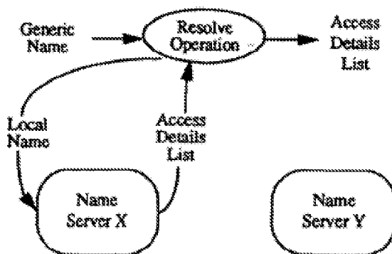
Figure 3: The Location Function
