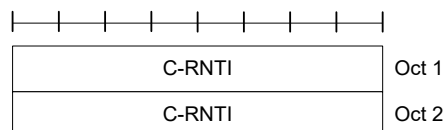
Figure 6.1.3.2-1: C-RNTI MAC control element
