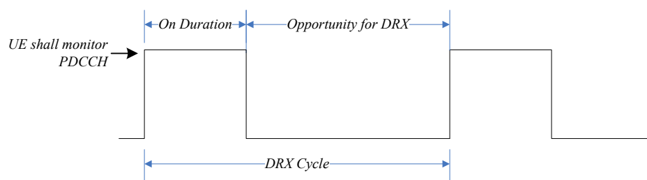
Figure 3.1-1: DRX Cycle
