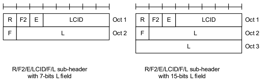
Figure 6.1.2-1: R/F2/E/LCID/F/L MAC subheader
