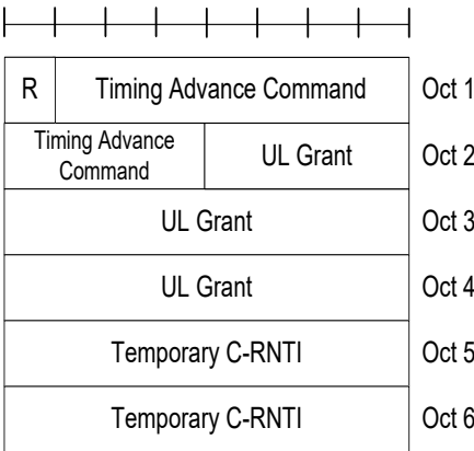
Figure 6.1.5-3: MAC RAR
