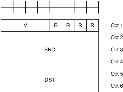
Figure 6.1.6-3: SL-SCH MAC subheader
