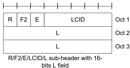
Figure 6.1.2-1a: R/F2/E/LCID/L MAC subheader
