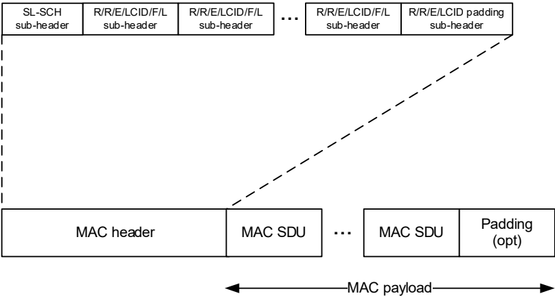
Figure 6.1.6-4: Example of MAC PDU consisting of MAC header, MAC SDUs and padding
