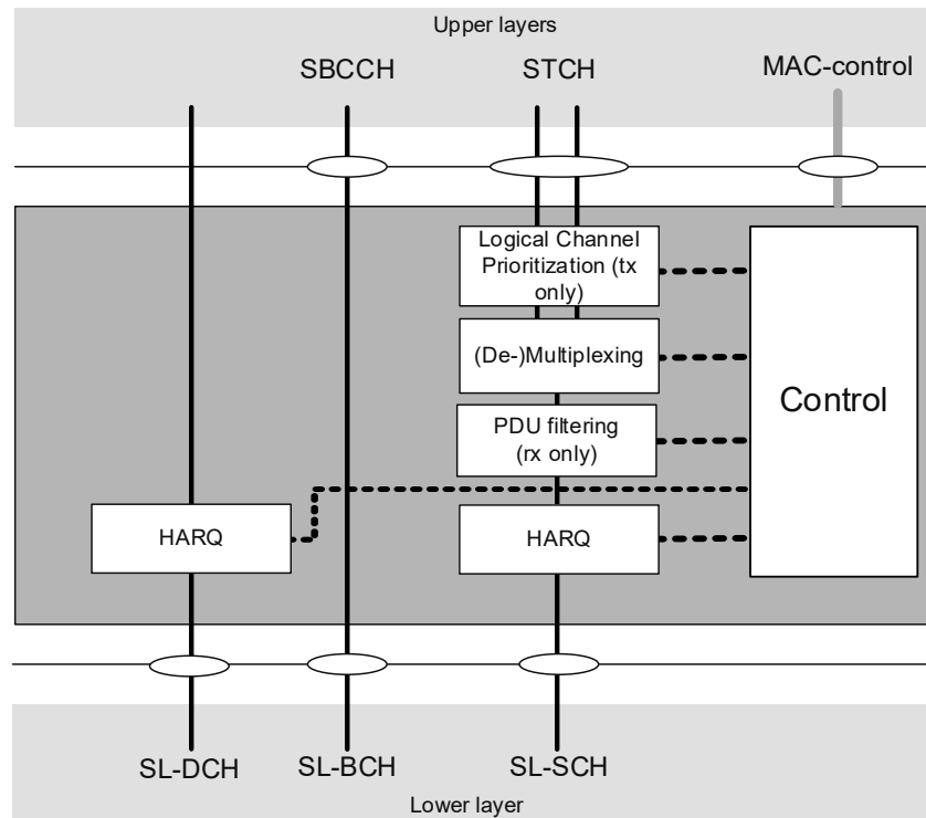
Figure 4.2.1-3: MAC structure overview for sidelink, UE side
