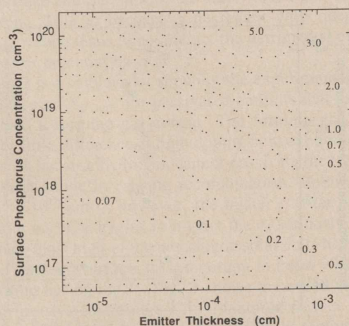
Fig. 6. Contours of constant J_0 for oxide-passivated emitters with a Gaussian phosphorus profile. The dependence of s versus N_{D, \text{surf}} used is the fit shown in Fig. 4, which was experimentally determined for emitters with an untextured surface, oxidized at 1000°C with no TCA, and with an FGA. The contours are labeled with the corresponding value of J_0 , in units of 10^{-13} \text{ A/cm}^2 .
