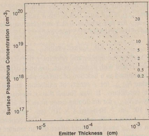
Fig. 8. Contours of constant J_{\text{lost}} for oxide-passivated emitters with a Gaussian phosphorus profile. J_{\text{lost}} is the photogenerated current density that is lost due to recombination in the emitter. The dependence of s versus N_{D,\text{surf}} used is the fit shown in Fig. 4, which was experimentally determined for emitters with an untextured surface, oxidized at 1000°C with no TCA, and with an FGA. J_{\text{lost}} was calculated for the SERI AM1.5 direct normal solar spectrum incident on the cell, normalized to have an incident intensity of 0.100 W/cm 2 (one sun). The photogenerated current density in 0.1 cm of silicon is 0.0415 A/cm 2 for this spectrum. The contours are labeled with the corresponding value of J_{\text{lost}} , in units of 10^{-13} A/cm 2 .
