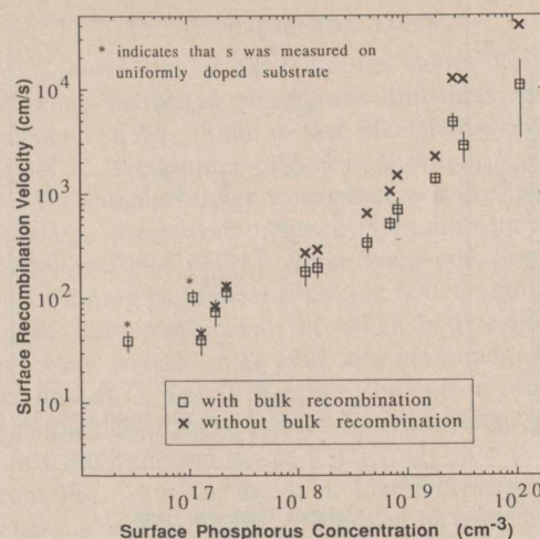
Fig. 5. Surface recombination velocity s extracted for both the standard case, in which the bulk recombination in the passivated emitter is accounted for, and the case in which there is no bulk recombination. The latter case gives an upper limit for s .
