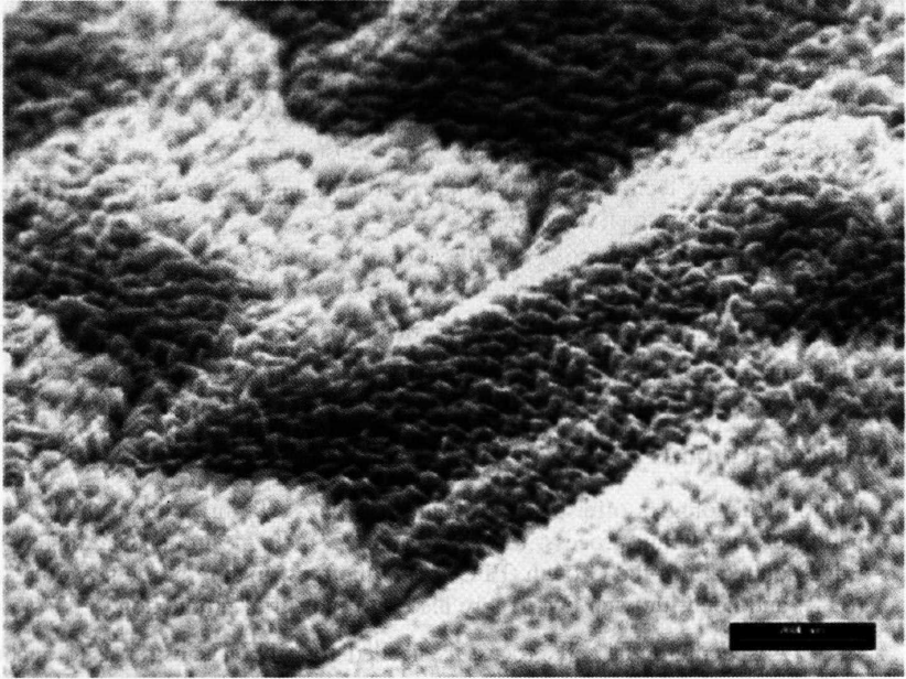
Figure 7.13 Mc-Si surface after RIE. (Reprinted from Solar Energy Materials and Solar Cells , 74, Szulcick J, Duerinckx F, Horzel J, Van Kerschaver E, Dekkers H, De Wolf S, Choulat P, Allebe C and Nijs J, "High-efficiency low-cost integral screen-printing multicrystalline silicon solar cells", 155–164, (2002), with permission from Elsevier Science)
