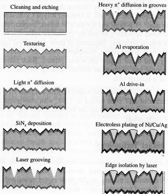
Figure 7.16 Laser-grooved buried-grid solar cell process
