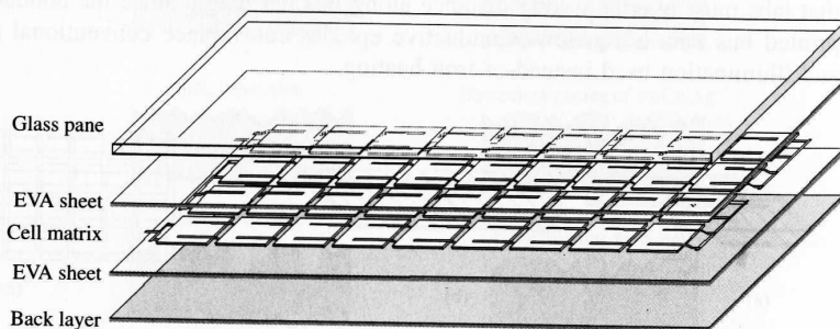
Figure 7.18 Stack of materials to be laminated
