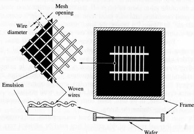
Figure 7.8 A screen for transferring the top contact pattern to a solar cell
