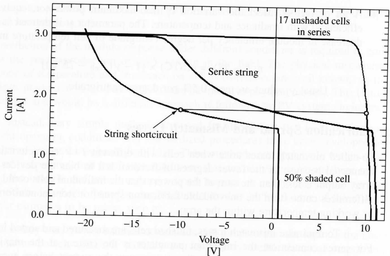
Figure 7.20 Computer simulation of the I-V curves of a 50% shaded cell, showing the typical “soft” reverse breakdown, and of 17 identical cells, unshaded, in series. When series-connected with the shaded cell, the curve labeled “series string” is obtained
