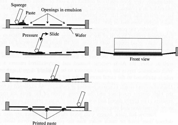
Figure 7.9 Illustration of a printing sequence
