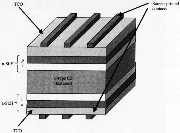
Figure 7.14 Structure of the HIT cell
