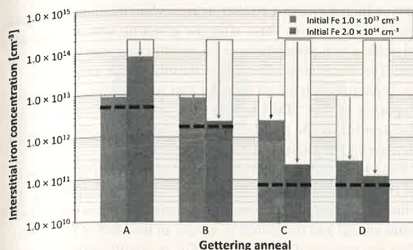
Fig. 1. Measured interstitial iron concentration in the bulk after different gettering anneals. The error estimate of the interstitial iron concentration value is \pm 2\% when iron concentration is below 1 \times 10^{12} \text{ cm}^{-3} and \pm 4\% when iron concentration is above 1 \times 10^{12} \text{ cm}^{-3} . The solid solubility of iron at the gettering anneal temperature [14], [15] is marked with a dotted line.
