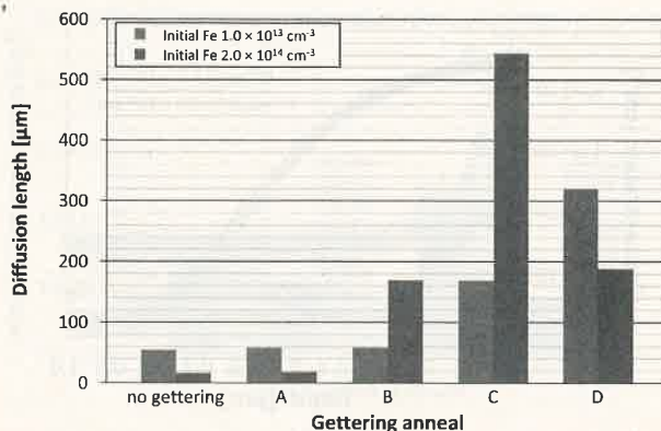
Fig. 2. Measured minority carrier diffusion length prior to dissociating the \text{Fe}_i\text{B}_s -pairs in the same samples as in Fig. 1.
