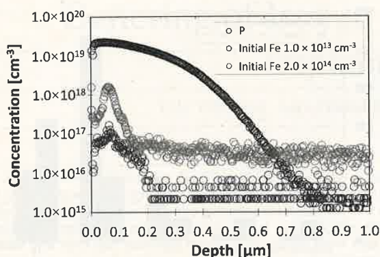
Fig. 3. Phosphorus and iron profiles near the wafer surface measured by SIMS from the high-Fe and medium-Fe wafers after gettering anneal C.
