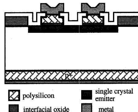
Figure 1. Cross section of the polysilicon BSF cells.
