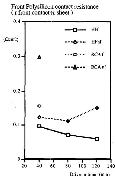
Figure 5. Specific resistance associated to the emitter.
