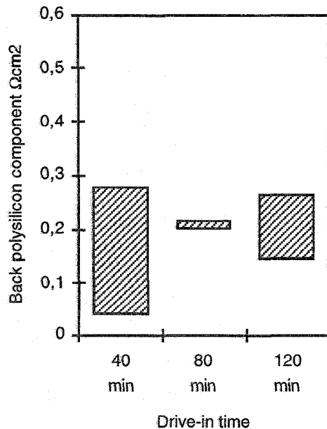
Figure 6. Specific resistance of the back contact structure.
