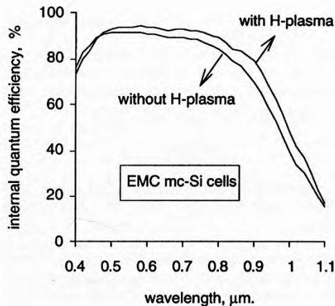
Figure 6. Internal quantum efficiency (IQE) of two RTP EMC mc-Si cells showing the effect of hydrogen plasma passivation
