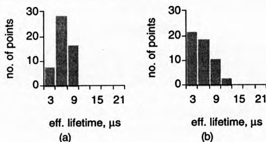
Figure 4. Distribution of \tau_{eff} in EMC mc-Si, (a) before, and (b) after an RT co-diffusion of P/Al at 925°C, 60s. (junctions were removed after RTD).
