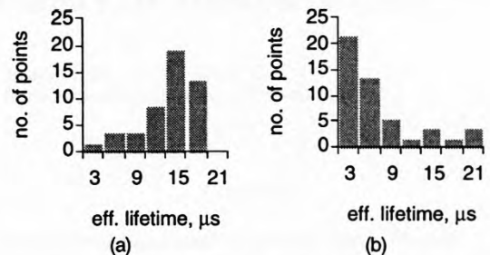
Figure 1. Distribution of \tau_{\text{eff}} in CC mc-Si, (a) before, and (b) after an RTA treatment of 925^\circ\text{C} , 60s, without involving any dopant diffusion
