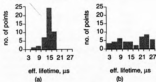
Figure 3. Distribution of \tau_{eff} in CC mc-Si, (a) before, and (b) after an RT co-diffusion of P/Al at 925°C, 60s. (junctions were removed after RTD).
