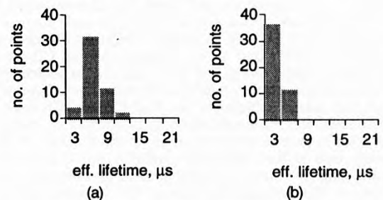
Figure 2. Distribution of \tau_{\text{eff}} in EMC mc-Si, (a) before, and (b) after an RTA treatment of 925^\circ\text{C} , 60s, without involving any dopant diffusion
