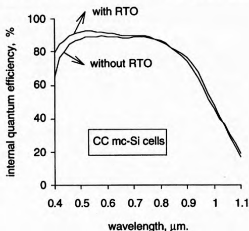
Figure 5. Internal quantum efficiency (IQE) of two RTP CC mc-Si cells showing the effect of RTO surface passivation
