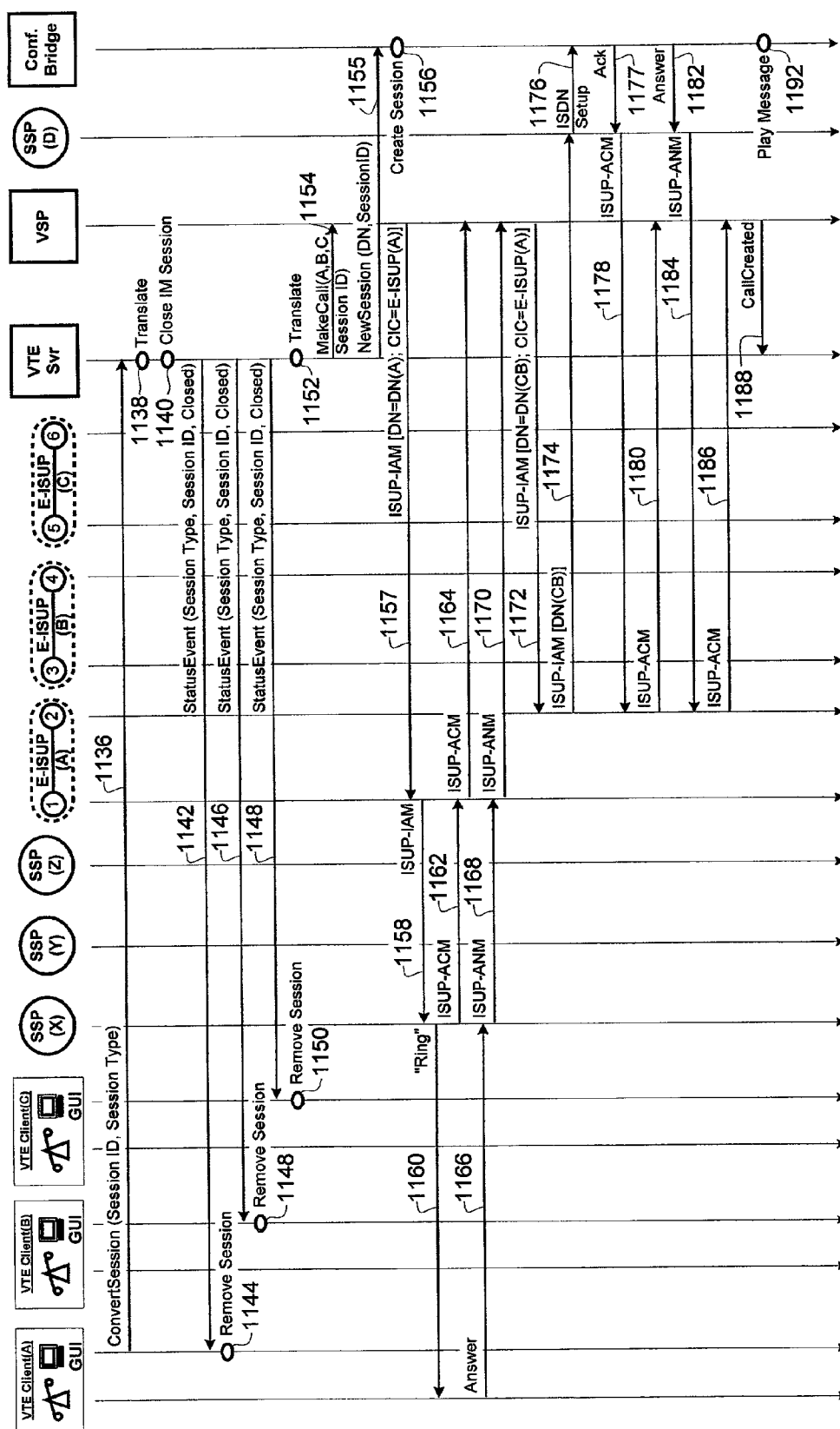
FIG. 32 Convert 3-Way IM Session to 3-Way Voice Communications Session
