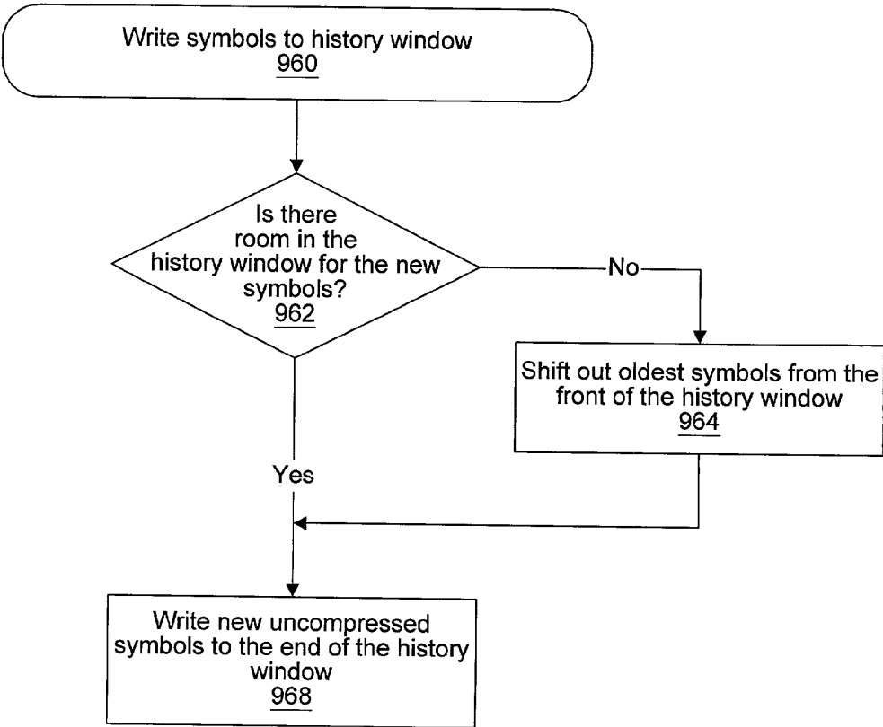
Decompression flowchart Fig. 23f
