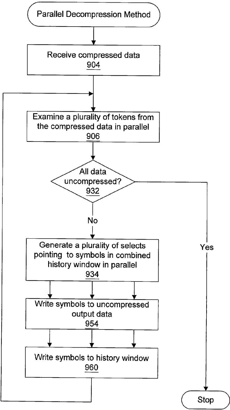
Decompression flowchart Fig. 23b
