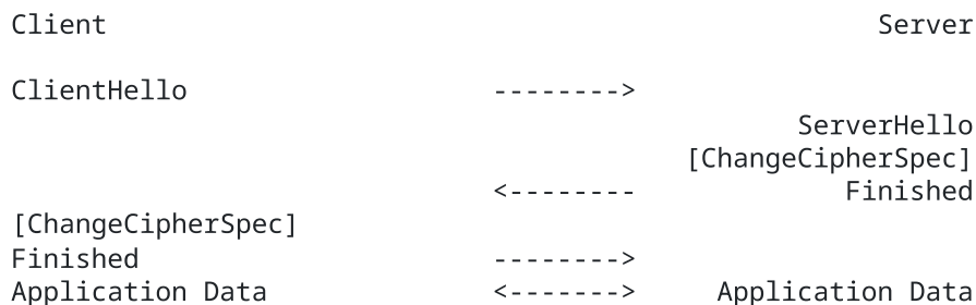
Figure 2. Message flow for an abbreviated handshake
