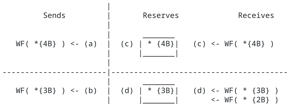
Figure 8: WF Reservation Example -- Partial Routing
