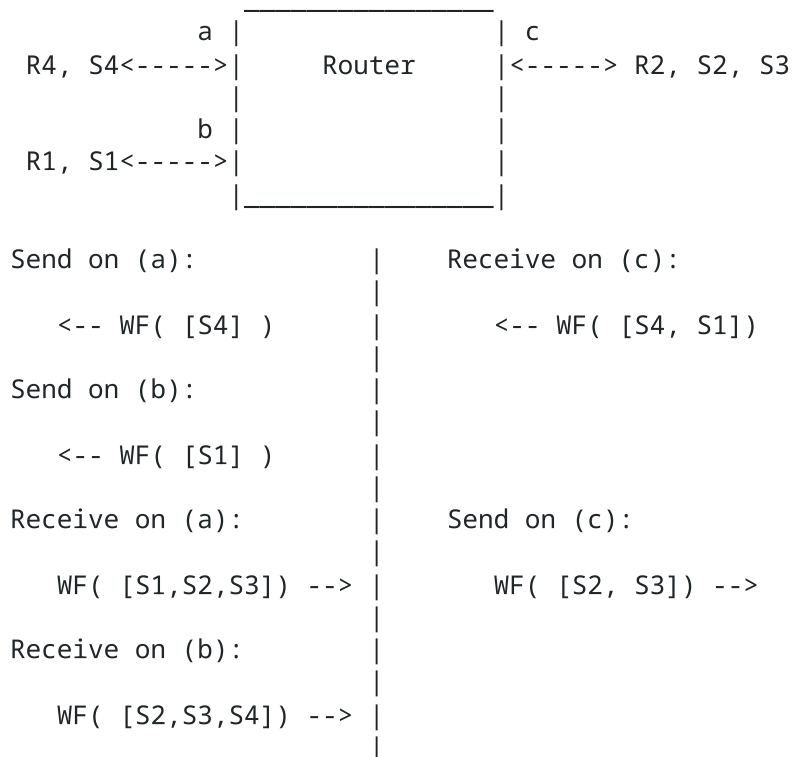
Figure 11: SCOPE Objects in Wildcard-Scope Reservations
