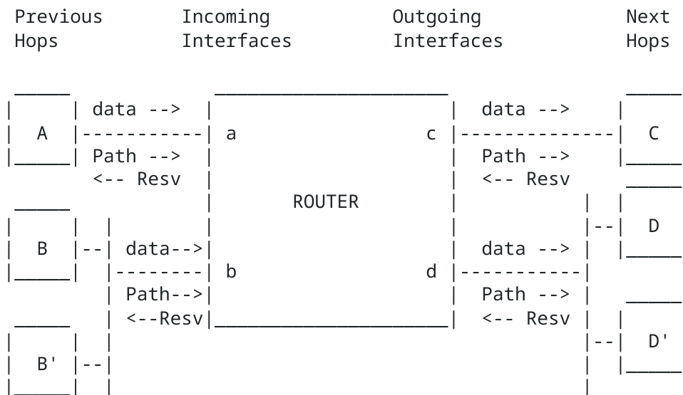
Figure 9: Router Using RSVP
