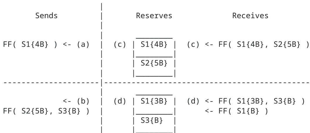
Figure 6: Fixed-Filter (FF) Reservation Example
