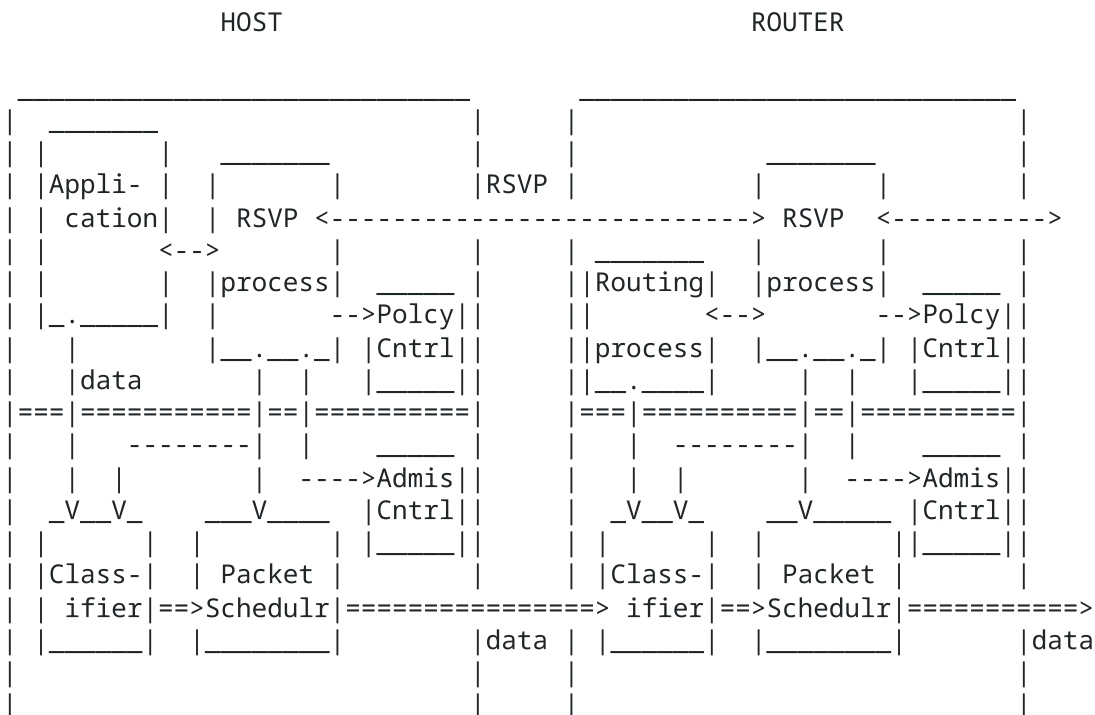
Figure 1: RSVP in Hosts and Routers
