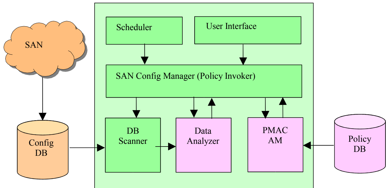
Figure 3 Extended SAN configuration manager
