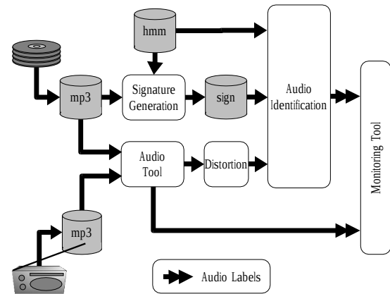
Figure 3. Test-bench schematic.
