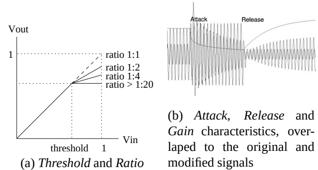
Figure 6. Compressor parameters
