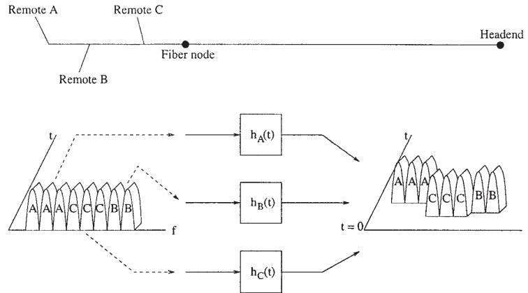
Figure 3: Example of multipoint-to-point DMT communications without synchronization
