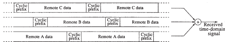
Figure 4: Loss of well-defined cyclic prefix when unsynchronized remote terminal transmissions are allowed in multipoint-to-point configurations
