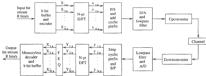
Figure 2: Passband DMT block diagram
