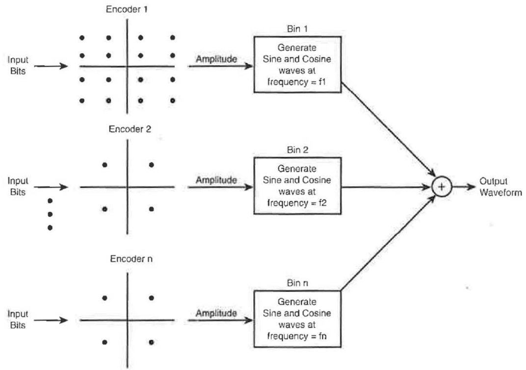
Conceptual view of a DMT modulator.
