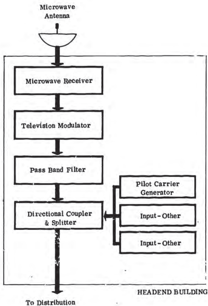
Figure 3-2: TYPICAL MICROWAVE HEADEND
