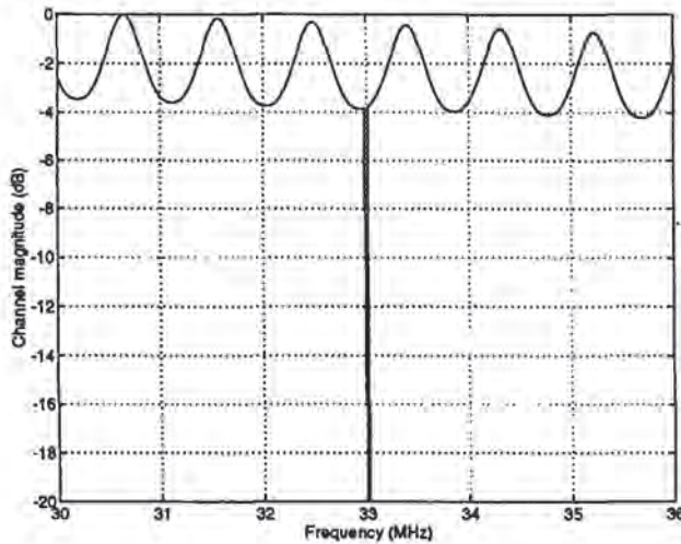
Figure 5: Frequency response magnitude of simulated channel with 30-kHz interferer
