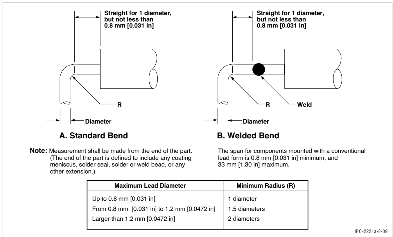
Figure 8-9 Lead Bends
