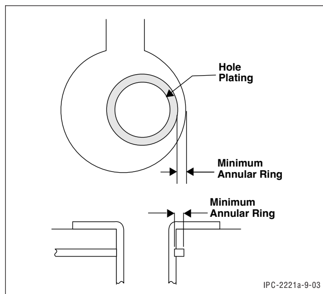
Figure 9-3 Internal Annular Ring
