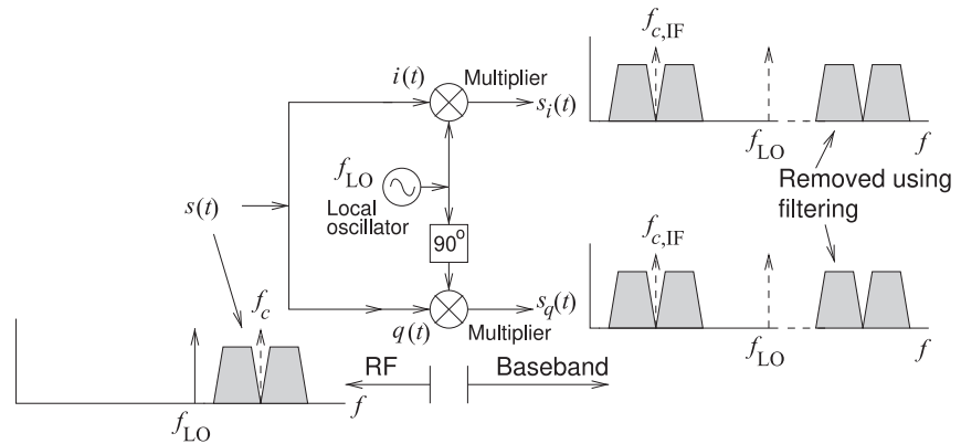
(b) Quadrature demodulator with f_{LO} < f_c , f_{c,IF} = f_c - f_{LO} .
