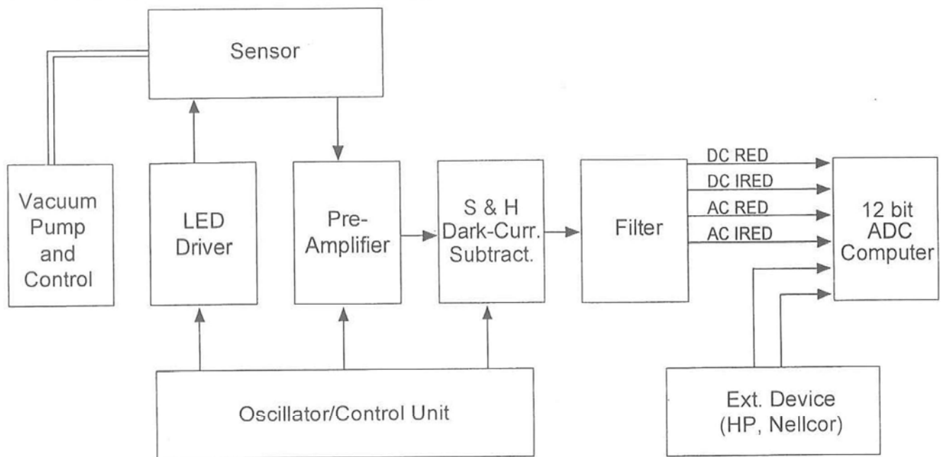
Fig. 2. Schematic representation of measurement electronics.
