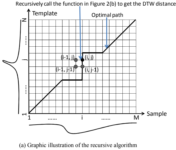
Figure 2: Dynamic Time Warping (DTW) algorithm to find the optimal matching between two time series
