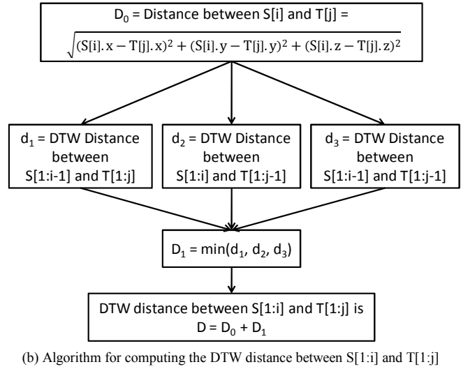
Figure 2: Dynamic Time Warping (DTW) algorithm to find the optimal matching between two time series
