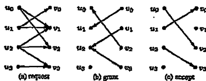
Figure 3: The three steps of a single iSLIP iteration.
