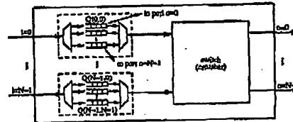
Figure 2: Schematic of a router using virtual output queuing.
