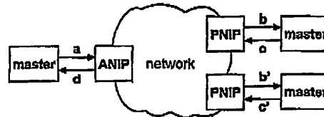
Figure 8. Message ordering is observable at a, b, c, and d.
