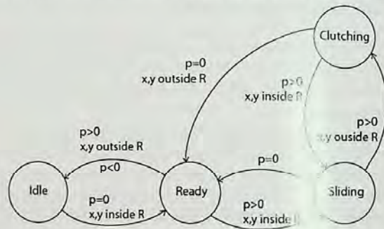
Figure 5: Zlider's state-transition diagram. R is the working rectangle; x,y the cursor's position. p<0 : stylus out of range; p=0 : stylus is being tracked; p>0 : stylus is touching the tablet. Zlider's scale is reset to 1 at the idle state
