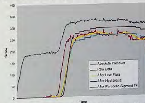
Figure 3: Effect of the stabilization techniques. The absolute pressure line represents the transducer's raw signal.
