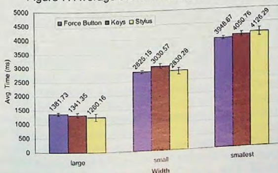
Figure 8: Average selection time per technique*width.
