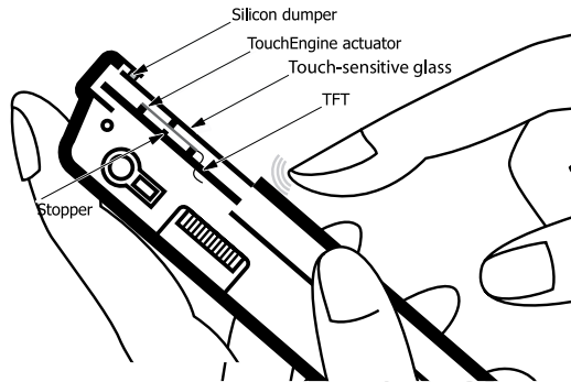
Figure 1: Haptic display for small touch screens.
