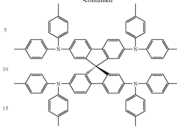
Spiro-TTB
