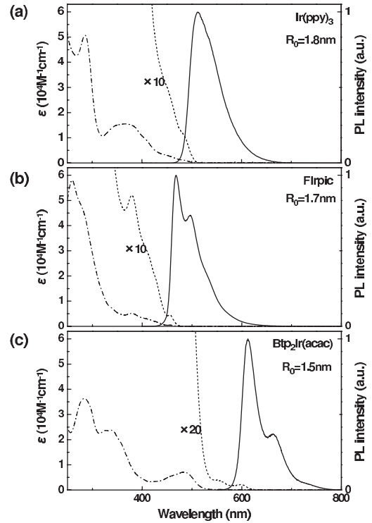
FIG. 3. Absorption (broken line) and PL spectra (solid line) of (a) \text{Ir(ppy)}_3 , (b) \text{Flrpic} , and (c) \text{Btp}_2\text{Ir(acac)} in methylenechloride ( 2 \times 10^{-5} M). The dotted lines show the absorption value expanded 10 times for the \text{Ir(ppy)}_3 and \text{Flrpic} and 20 times for the \text{Btp}_2\text{Ir(acac)} . The Förster radii ( R_0 ) obtained by the spectral overlap in Eq. (3) are shown.
