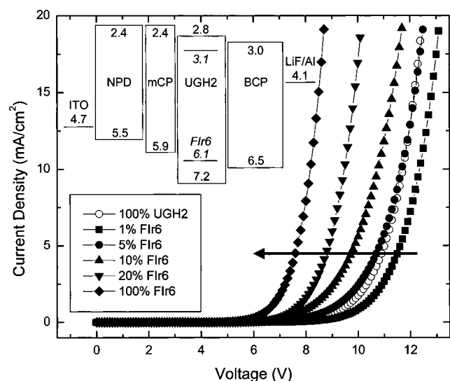
FIG. 4. J - V characteristics for ITO/NPD (40 nm)/mCP (15 nm)/UGH2: x % Fir6 (25 nm)/BCP (40 nm)/LiF (0.5 nm)/Al (50 nm) OLEDs. The arrow points in the direction of increasing Fir6 concentration. Inset: Proposed energy level scheme for the device under zero applied bias.
