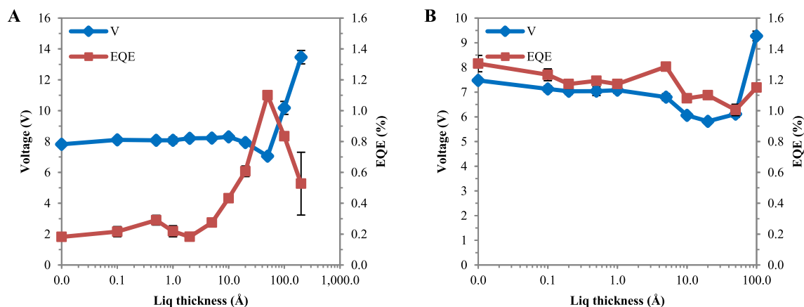
Fig. 1. Drive voltage and EQE dependence on Liq thickness for devices: (A) ITO|MoO x (20 Å)|NPB(600 Å)|Alq 3 (400 Å)|Liq(x)|Ag, and (B) ITO|MoO x (20 Å)|NPB (600 Å)|Alq 3 (400 Å)|Bphen (100 Å)|Liq(x)|Ag. The voltage and EQE were measured at 20 mA/cm 2 .
