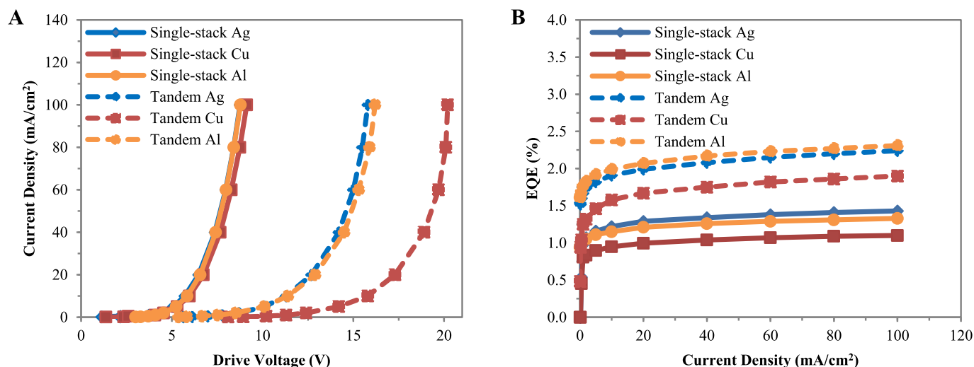
Fig. 5. Current density-voltage (A) and current density-external quantum efficiency (B) characteristics for two-stack tandem devices: ITO|MoO x (20 Å)|NPB (600 Å)|Alq 3 (400 Å)|Bphen (100 Å)|LiQ (40 Å)|Metal (40 Å)|MoO x (20 Å)|NPB (600 Å)|Alq 3 (400 Å)|Bphen (100 Å)|LiQ (20 Å)|Ag.
