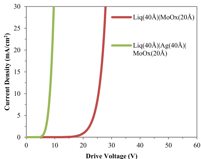
Fig. 4. Current density-voltage characteristics for: ITO|Alq 3 (400 Å)|Bphen (100 Å)|EIL|MoO x (20 Å)|NPB(600 Å)|Ag devices, where the EIL is 1) Liq (40 Å)|Ag (40 Å) and 2) Liq (40 Å).
