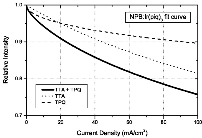
FIG. 14. Solid line: model calculation of the NPB:Ir(piq) 3 based OLED. The other two curves are generated by ignoring one or the other quenching process. The plot is on linear scale for better visibility.
