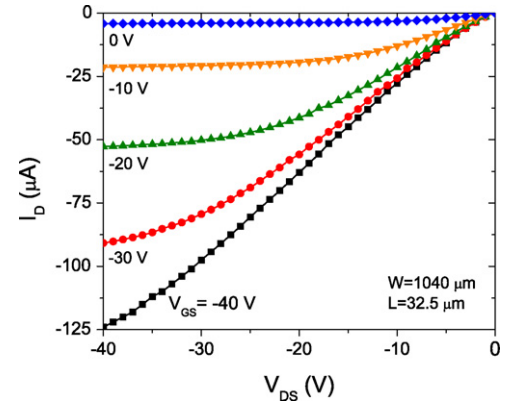
Fig. 8. Output characteristics of a CuTBP OFET.
