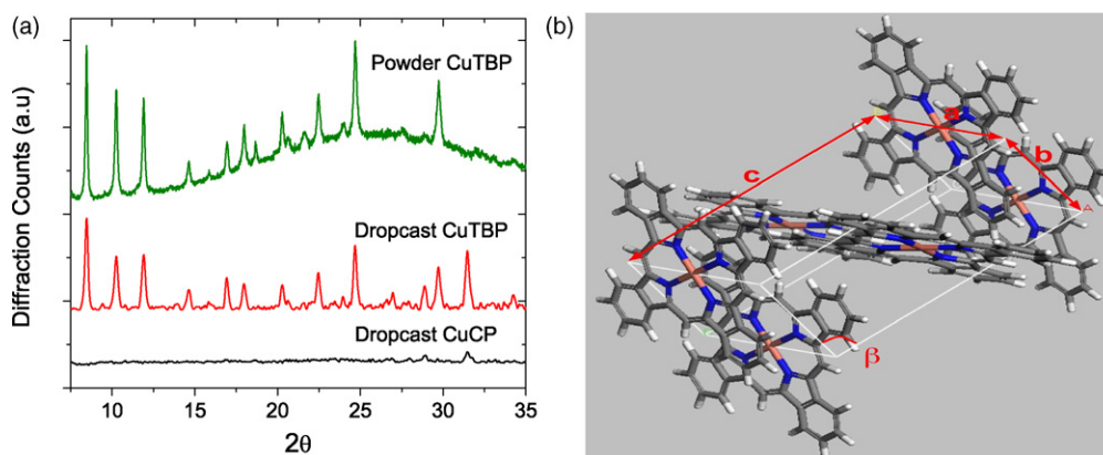
Fig. 3. (a) X-ray diffraction spectra for drop-cast CuCP and CuTBP, and powder CuTBP, and (b) the proposed unit cell structure of solid CuTBP.
