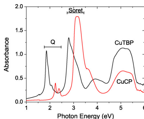
Fig. 6. Optical absorbance spectra for spun-cast CuCP and CuTBP thin-films on quartz.
