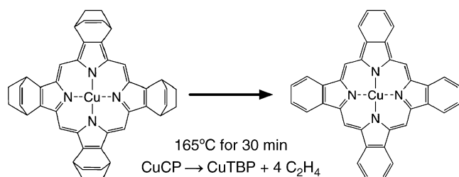
Fig. 1. Thermal conversion of CuCP to CuTBP.
