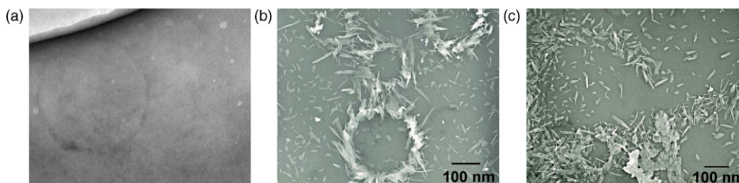
Fig. 5. TEM micrographs of: (a) precursor CuCP, (b) sparse CuTBP, and (c) more dense CuTBP with parallel aggregation, drop-cast onto Cu grids coated with amorphous carbon.
