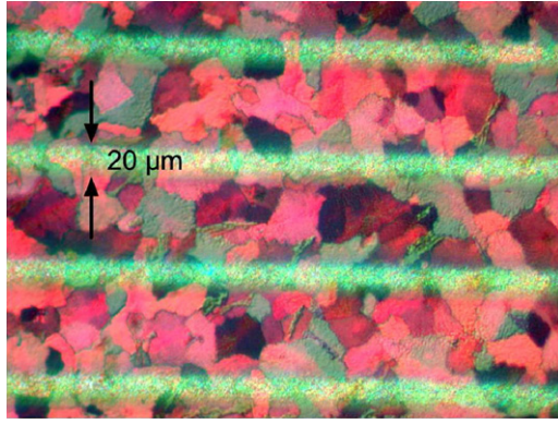
Fig. 7. Polarized optical micrograph of a continuous, spun-cast CuTBP thin-film on thermally oxidized c-Si. The electrodes shown in the figure are 20 \mu\text{m} wide. Color variations in the film indicate individual nanorod domains. (For interpretation of the references to color in this figure legend, the reader is referred to the web version of the article.)
