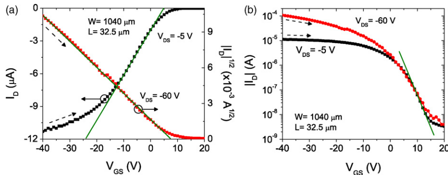
Fig. 9. Transfer characteristics of a CuTBP OFET. Dashed arrows indicate the measurement direction. In (a), the solid lines indicate the fits to Eqs. (1) and (2); in (b), the solid line indicates calculation of the subthreshold slope.
