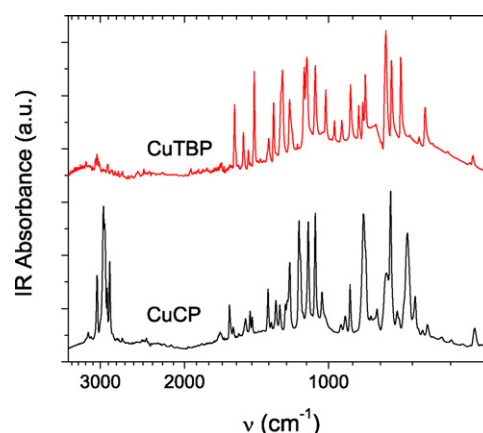
Fig. 2. Infrared absorbance spectra for solid CuCP and CuTBP on c-Si.
