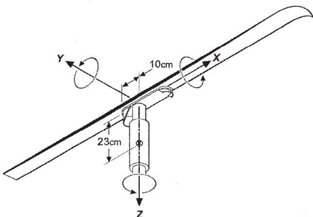
FIG. 2 Test Equipment
