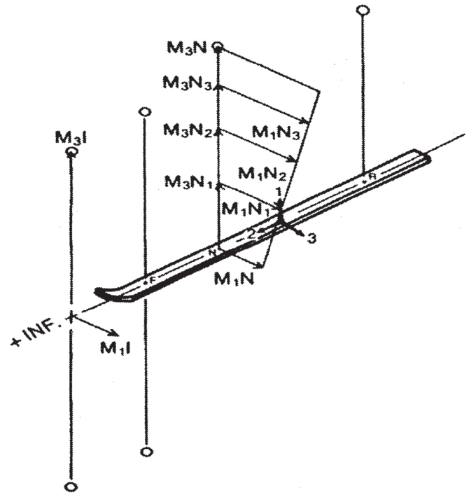
FIG. X1.3 Partial Release Envelope Showing Release Moments in Twist Under Combined Loading Using a Preload in Forward Lean 24
