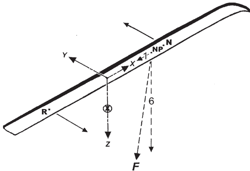
FIG. A1.3 Release with Combined Loading Test
