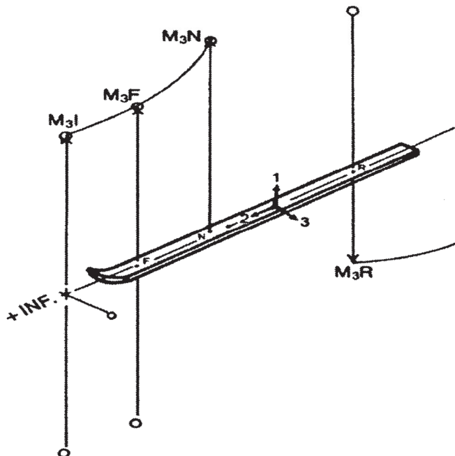
FIG. X1.2 Partial Release Envelope Showing Release Moments in Forward Lean 23
