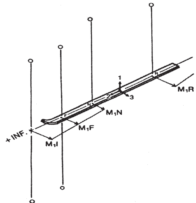
FIG. X1.4 Partial Release Envelope Showing Release Moments in Twist 25
