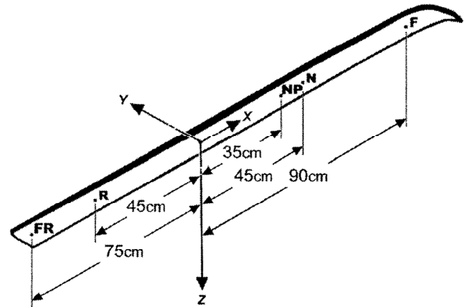
FIG. 1 Load Application
