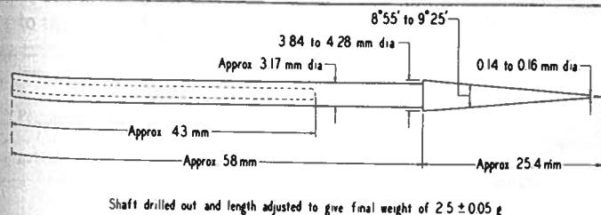
FIG. 2 Standard Needle
