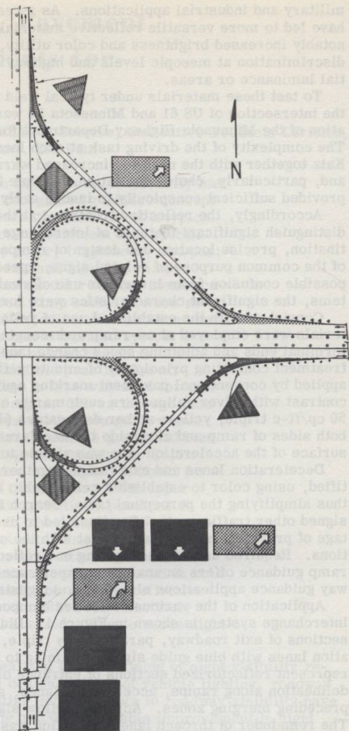
Figure 1. A unified reflective sign, delineator and roadway color treatment showing order of presentation for northbound traffic through a typical interchange. Similar systems may be employed in a number of related traffic guidance applications.
