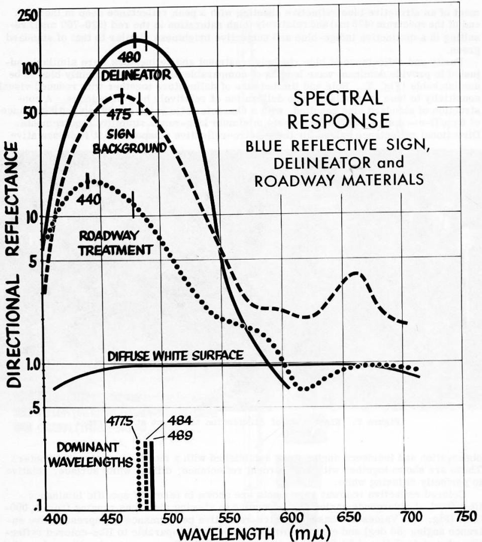
Figure 3. Spectral distribution of blue reflective signs, delineators and roadway marking materials shown relative to a diffuse white surface. Figures for spectral response at peak reflectance and dominant wavelength are given in millimicrons.
