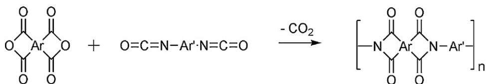
Scheme 44. Synthesis of polyimides from diisocyanates and dianhydrides.
