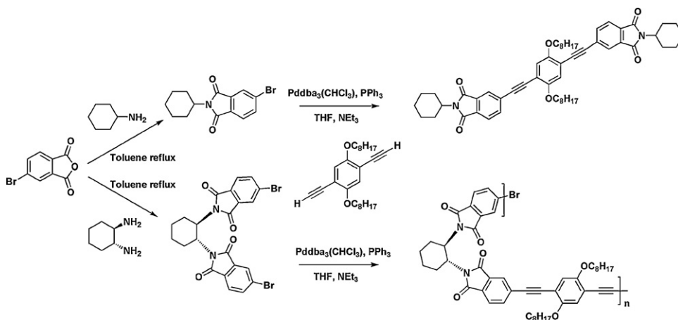
Scheme 66. Phenyleneethynylene-based polyimide which combines the C2 chiral structure with a confined chromophore [361].
