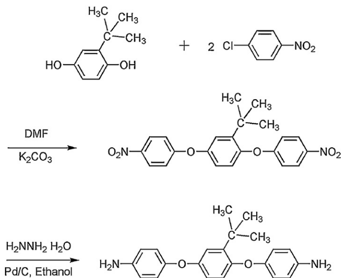
Scheme 15. Unsymmetrical ether-containing diamines.
