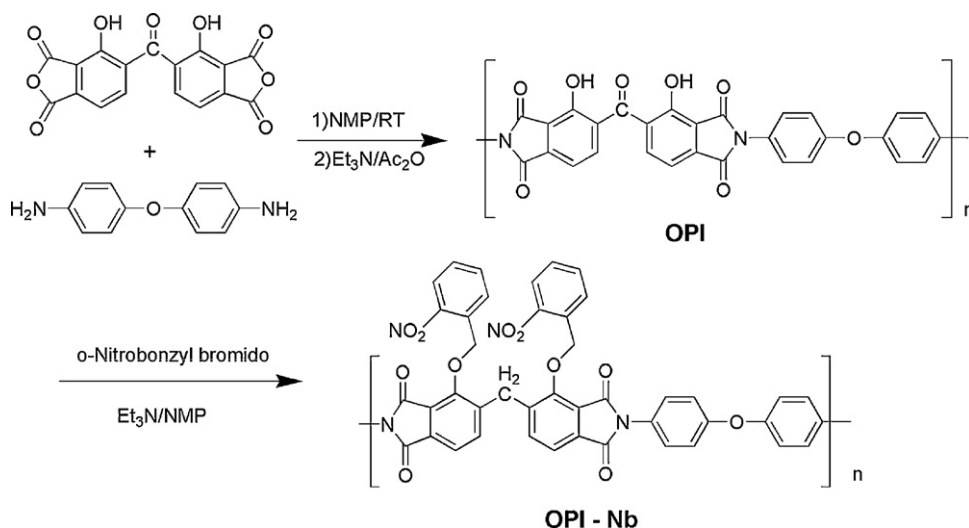
Scheme 53. Synthetic route to photosensitive OPI-Nb.
