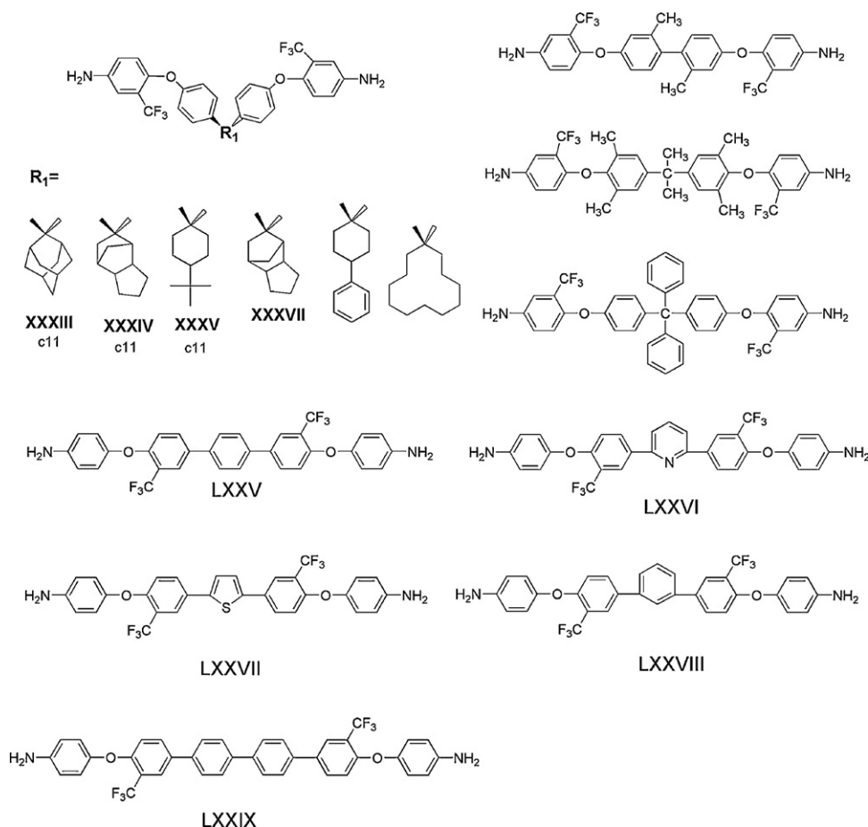
Scheme 21. Diamines containing trifluoromethyl with different linkages [87].
