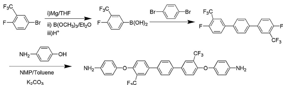
Scheme 22. Synthesis of monomer, LXXV [88].
