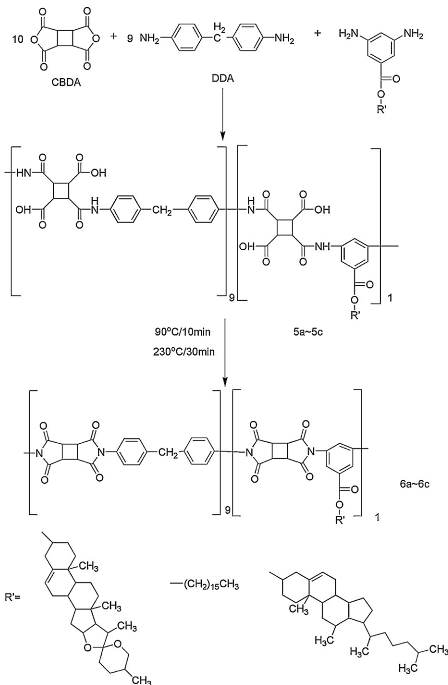
Scheme 58. Synthesis of the (poly(amic acid)s and the polyimides from CBDA and DDA [256].
