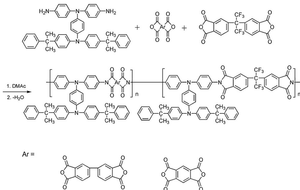
Scheme 73. Copolyimides with propeller-shaped triarylamine unit prepared from the diamine and various aromatic dianhydride via direct polycondensation [54].
