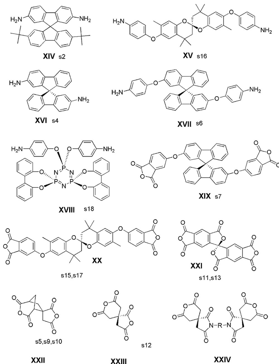
Scheme 6. Chemical structures of novel spiro diamines and dianhydrides.
