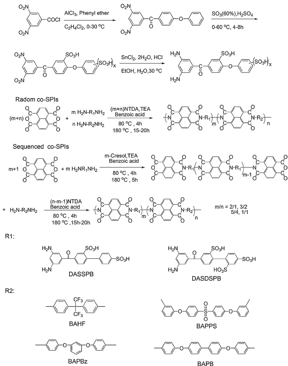
Scheme 35. Synthesis of diamine monomers with sulfonic acids at side chain [165].
