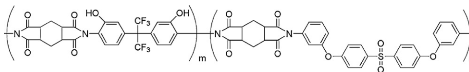
Scheme 51. Structure of Bco-PI.
