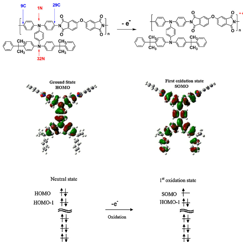
Scheme 74. Electrochromic mechanism and electronic density contours of polyimide 1b structure.
