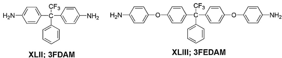
Scheme 19. Chemical structures of XLII (3FDAM) and XLIII (3FEDAM).
