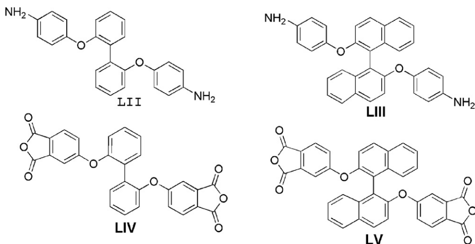
Scheme 9. Crank and twisted noncoplanar structure diamines or dianhydrides.
