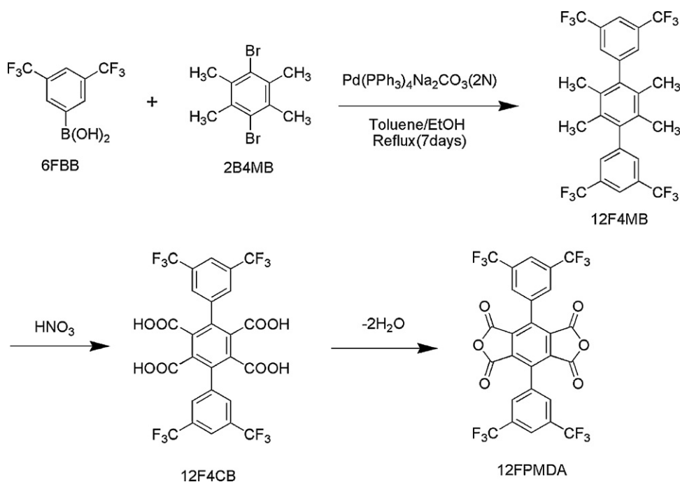
Scheme 25. Synthesis of 12FPPMDA [92].
