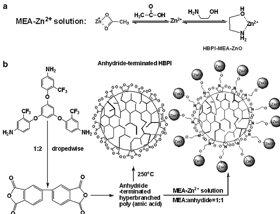
Scheme 76. Novel nano ZnO/hyperbranched polyimide hybrid [420].
