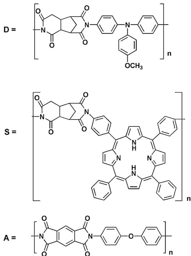
Scheme 62. Structures using triphenylamine unit as an electron donor (D), tetraphenylporphyrin as a sensitizer (S), and aromatic polyimide as an electron acceptor (A).
