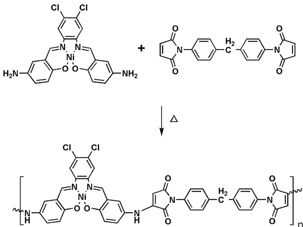
Scheme 46. Synthesis of polyimides from diamine and bis(maleimide).
