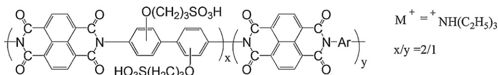
Scheme 69. Copolyimides bearing pendant sulfonic acid groups [375].
