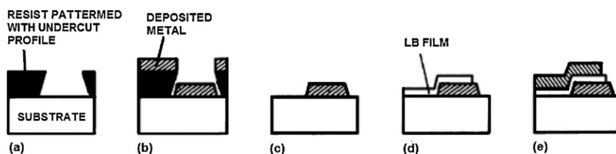
Fig. 2. Fabrication process of switching elements. (A) The resist is patterned with an undercut profile. (B) The base-electrode metal is deposited. (C) The excess metal is lifted off when the resist is removed, leaving behind a patterned deposit on the substrate surface. (D) The LB film is deposited. (E) The top-electrode metal is deposited and patterned using a conventional wet etching after the resist process.
