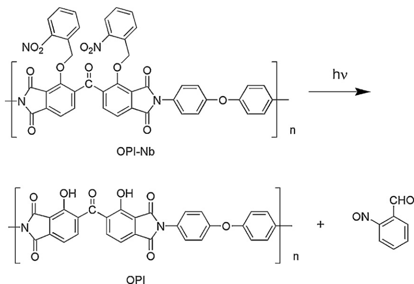
Scheme 54. Photochemical reaction of OPI-Nb.
