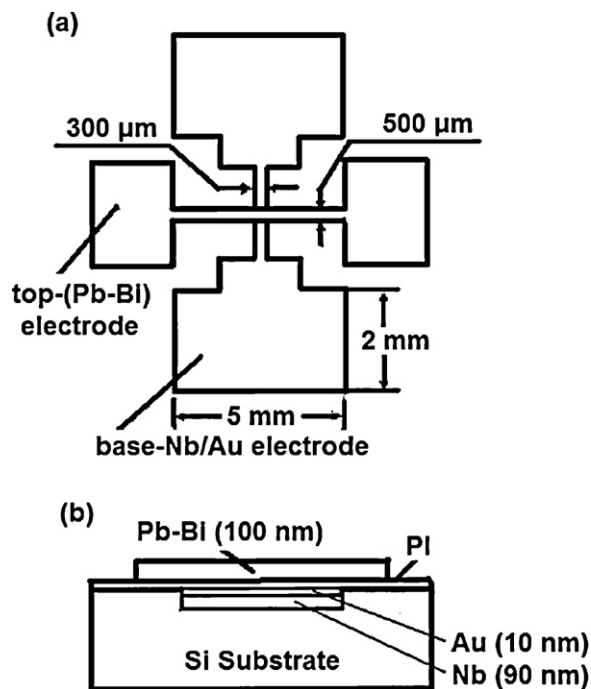
Fig. 1. Josephson junction (A) top view and (B) side view.
