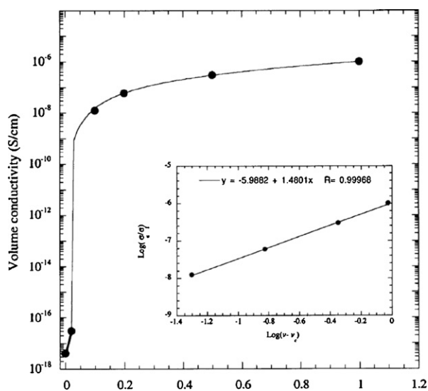
Fig. 5. Volume conductivity of SWNT-CP2 nanocomposites [407]. Copyright 2002, Elsevier Ltd.
