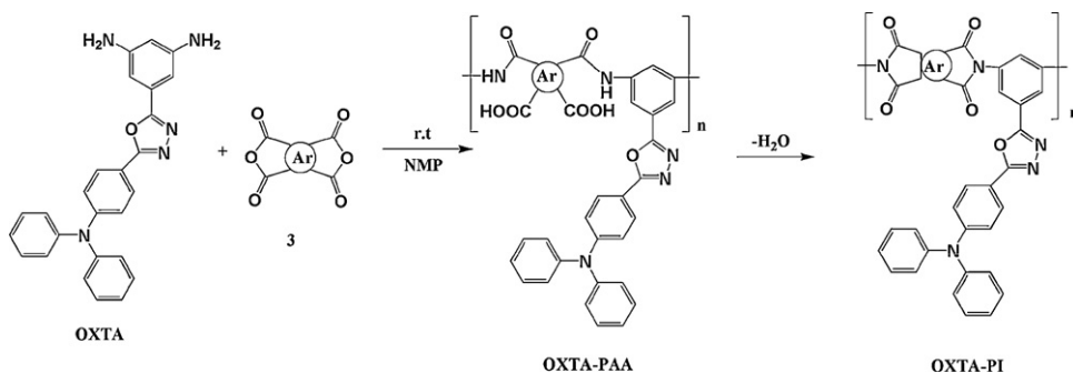
Scheme 79. Aromatic polyimides (OXTA-PI)s containing triphenylamine and 1,3,4-oxadiazole moieties [435].
