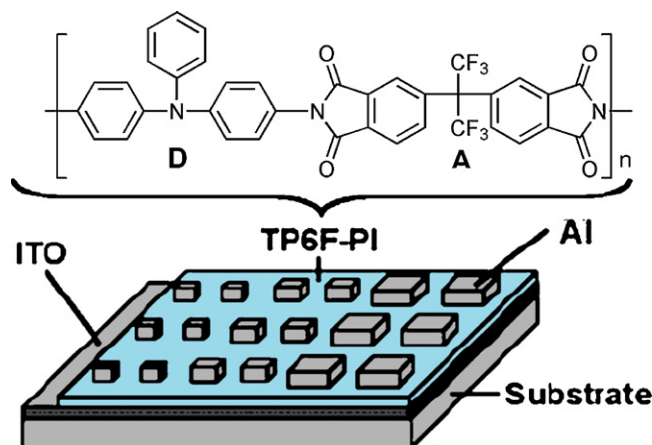
Scheme 78. Molecular structure and schematic diagram of the single layer memory device [437].
