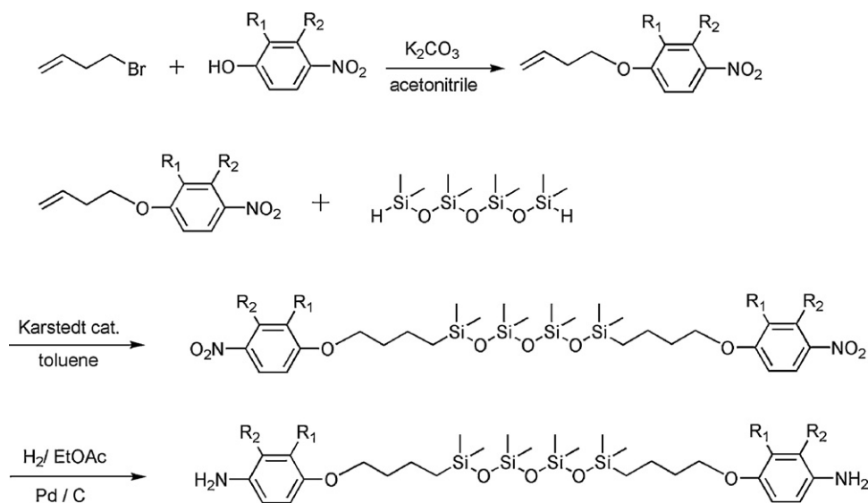
Scheme 59. Novel siloxane-containing liquid crystalline (LC) polyimides [257].
