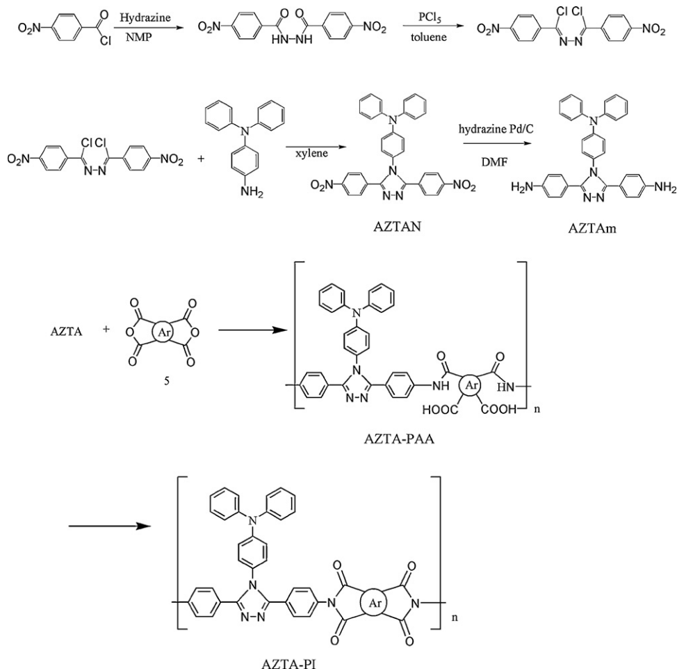
Scheme 80. Aromatic polyimides containing triphenylamine-substituted triazole moieties [436].
