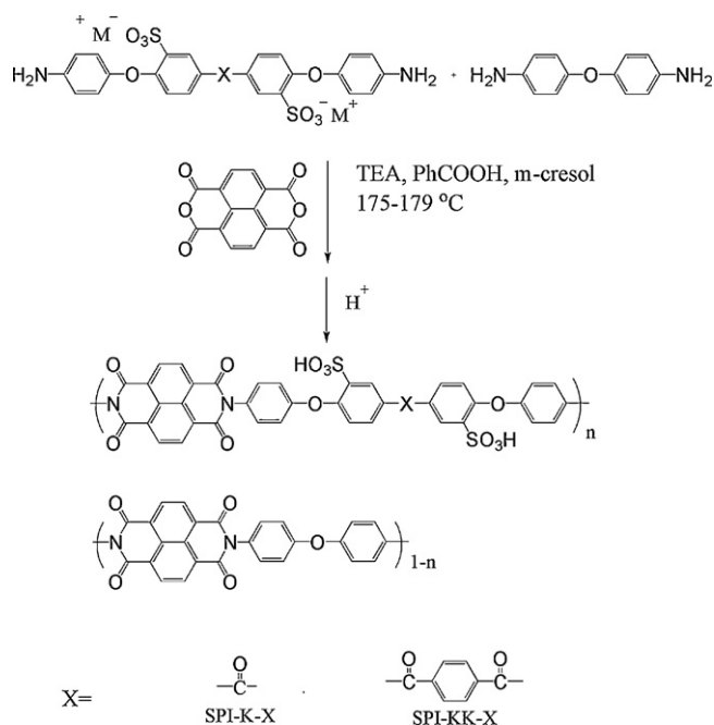
Scheme 70. SPIs containing ether and ketone linkages through a copolymerization method [383].
