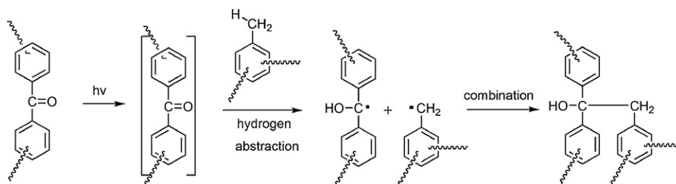
Scheme 57. Photocrosslinking of a benzophenone unit and alkyl moiety.
