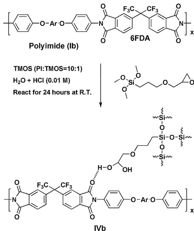
Scheme 61. Prepared series of new polymer–silica hybrid materials through the intrachain bonding by \gamma -glycidyloxypropyltrimethoxysilanes (GOTMS) [335].
