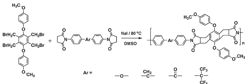
Scheme 47. Synthesis polyimide by Diels–Alder reaction.
