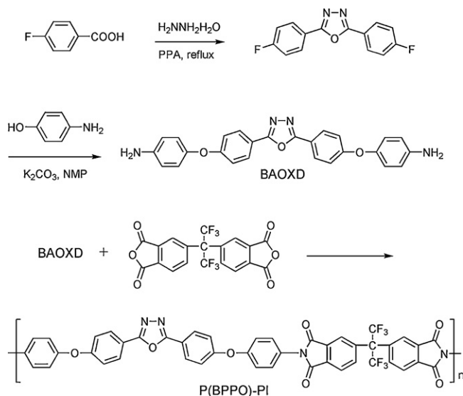
Scheme 81. Synthesis of functional polyimide, P(BPPO)-PI, containing oxadiazole moieties (electron donors) and phthalimide moieties (electron acceptors) [439].
