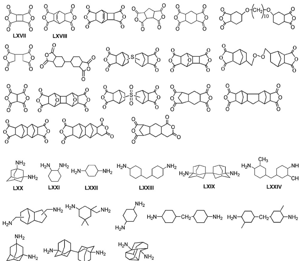
Scheme 16. Chemical structures of alicyclic monomers.
