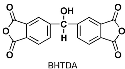
Scheme 5. Functional dianhydride ( BHTDA ) with a hydroxyl group.
