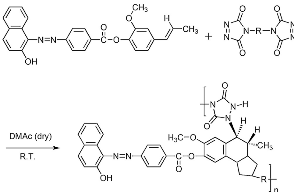
Scheme 27. Synthesis of novel heterocyclic polyimides containing the azo-naphthol pendant group via Diels–Alder-ene cycloaddition reactions from an azo-ester.
