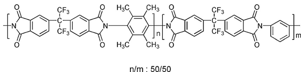
Scheme 60. Polyimide for gas separations.
