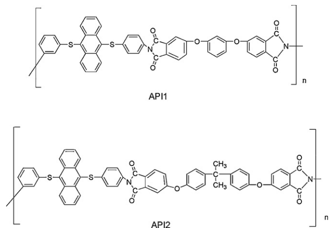
Scheme 63. Molecular structures of APIs [356,358].
