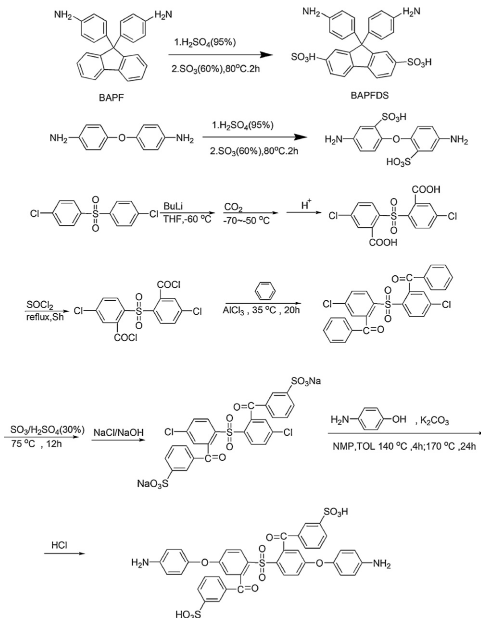
Scheme 32. Sulfonated diamines derived from sulfonation reaction [161–163].
