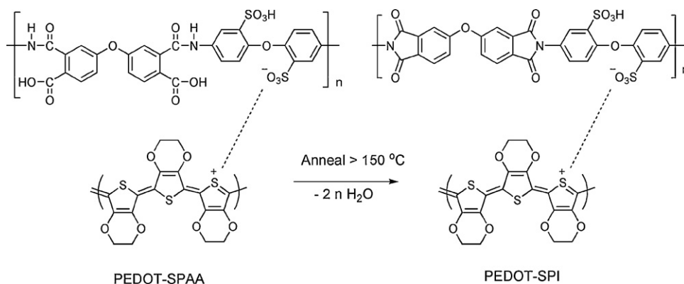
Scheme 71. PEDOT-SPI derived from PEDOT-SPAA [384].
