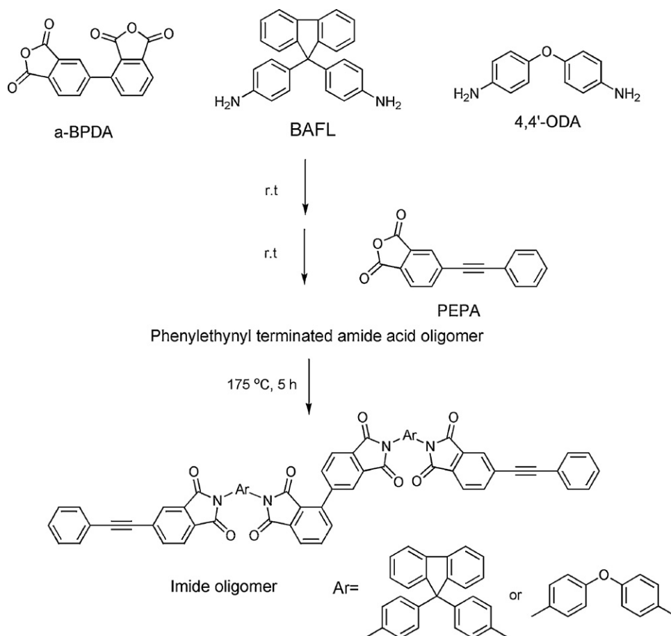
Scheme 83. Synthesis of the additive imide oligomers by Yokota and coworkers [440].
