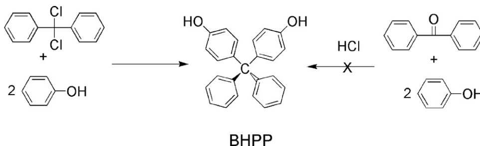
Scheme 3. Synthesis of BHPP.
