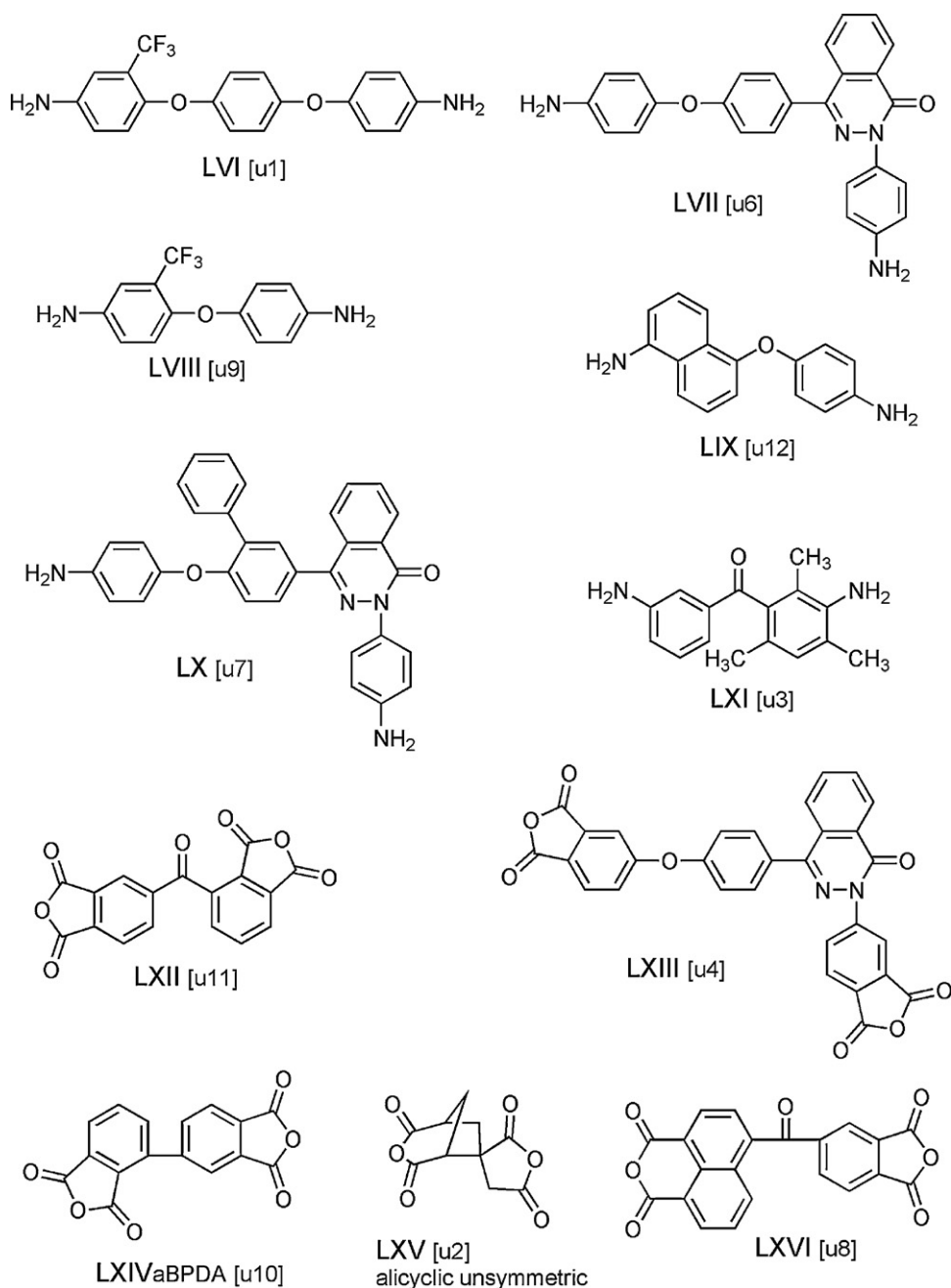
Scheme 11. Chemical structures of unsymmetric monomers.
