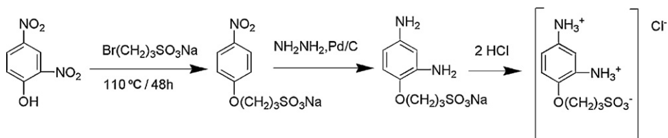
Scheme 34. Synthesis of sulfonated diamine monomer (DAPPS) [164].
