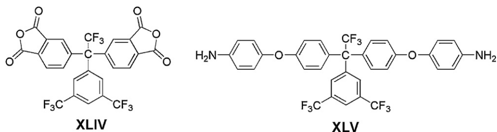
Scheme 20. Triarylfluoroethanes-containing dianhydride ( XLIV ) and diamine ( XLV ).
