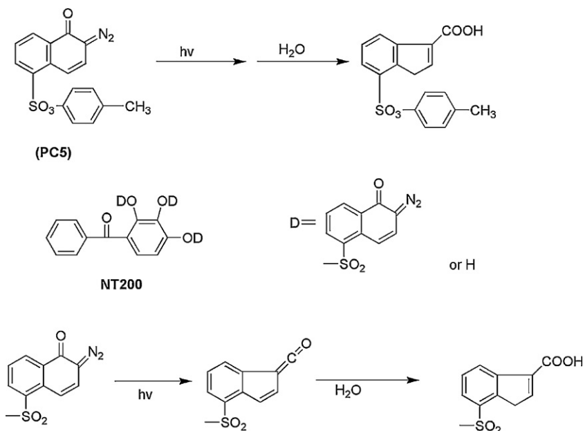
Scheme 52. Structures and reactions of photoreactive compounds under exposing and developing.
