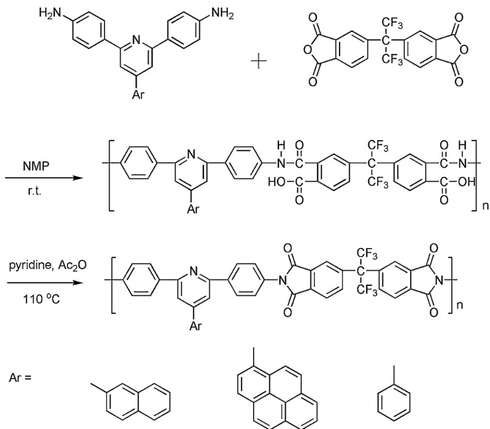
Scheme 43. Synthesized poly(pyridine-imide)s prepared by the conventional two-step polymerization method.
