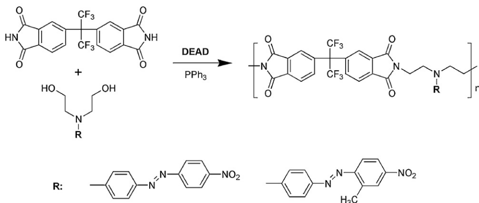
Scheme 40. NLO polyimide via (A) two-step and (B) one-step Mitsunobu condition [181].
