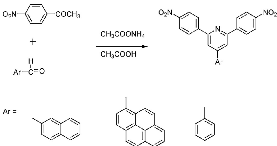
Scheme 28. Synthesis of pyridine-containing dinitro derived by Chichibabin.
