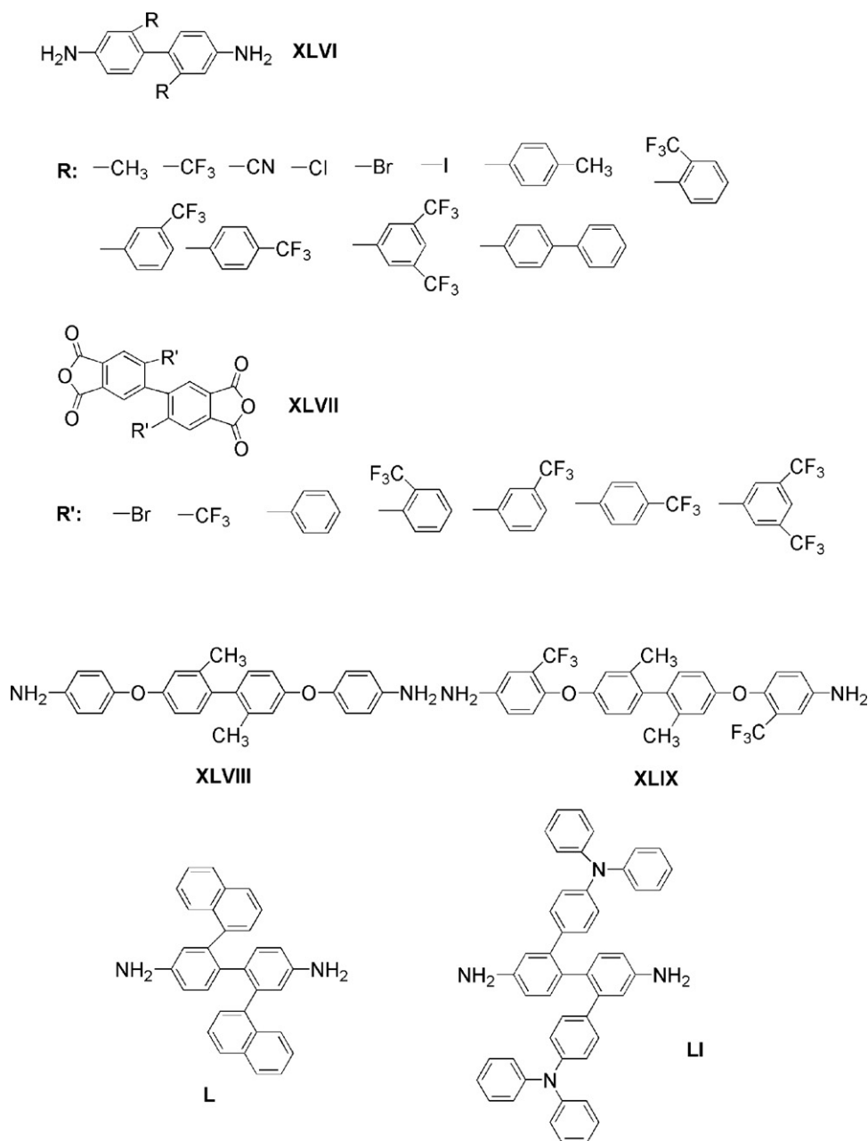
Scheme 8. Monomers with noncoplanar structure.
