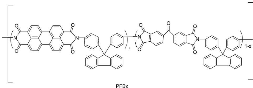
Scheme 65. Novel diphenylfluorene-based cardo copolyimide containing perylene (PFB5) [360].
