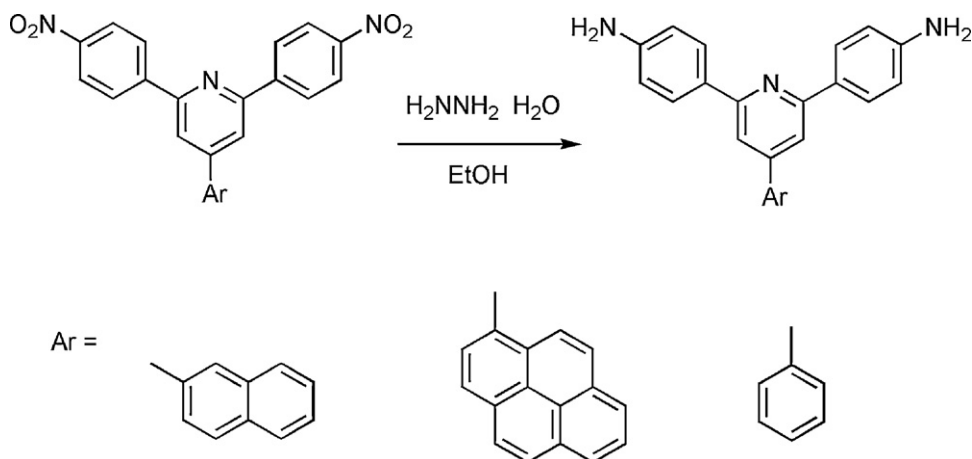
Scheme 29. Synthesis of pyridine-containing diamines.
