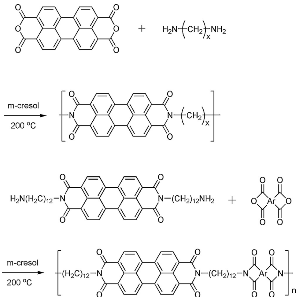
Scheme 31. Two most used approaches to preparing organo-soluble pyrene-containing polyimides.
