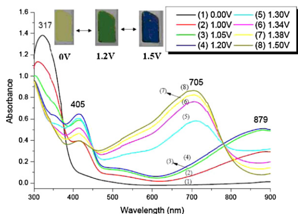
Fig. 3. Electrochromic behavior of polyimide 1b film (in \text{CH}_3\text{CN} with 0.1 M TBAP as the supporting electrolyte).
