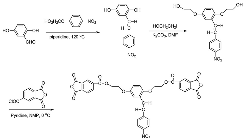
Scheme 37. Synthesis of T-shaped NLO dianhydride [172].
