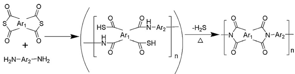
Scheme 45. Synthesis of polyimides from diamine and dithioanhydride.
