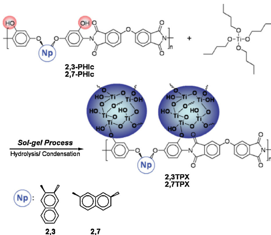
Scheme 77. Polyimide–nanocrystalline–titania hybrid synthesized from the hydroxy-substituted diamines with various commercial tetracarboxylic dianhydrides [421].
