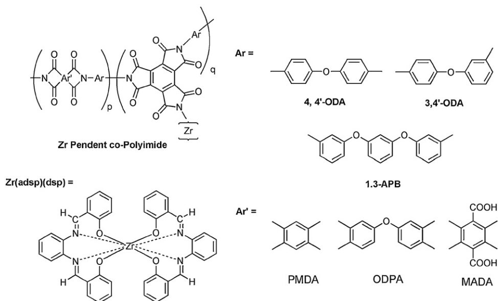
Scheme 41. Structures of dianhydrides, diamines, and pendent group, and structure of polyimide products.
