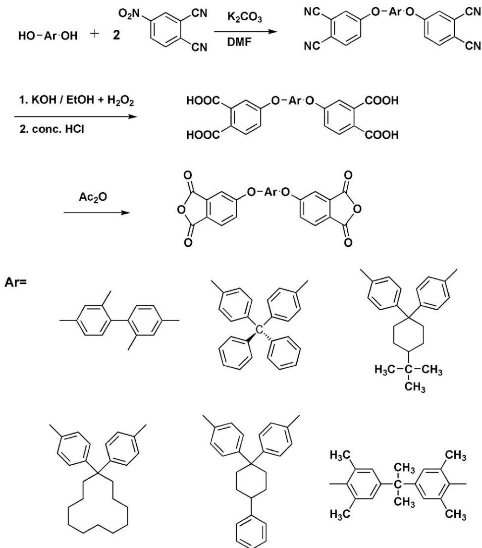
Scheme 4. Preparation of bis(ether anhydride)s.
