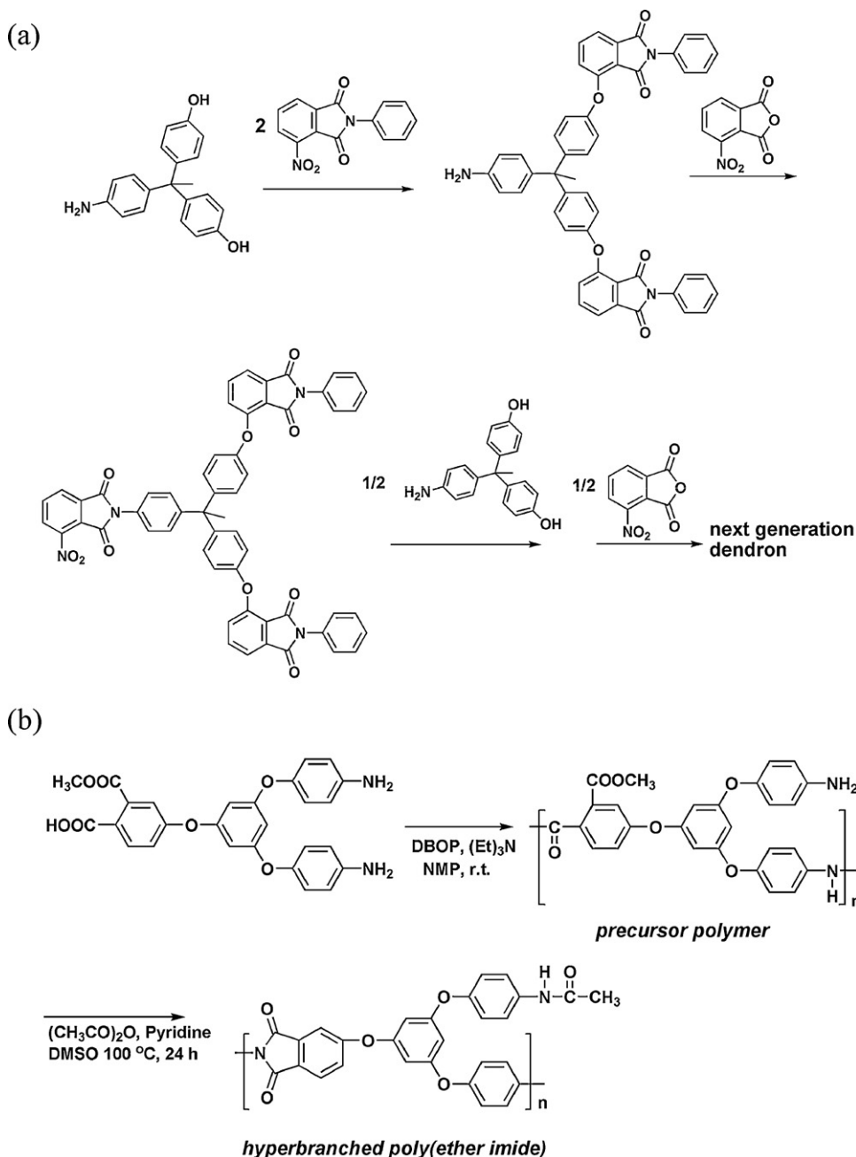
Scheme 49. (A) Preparation of dendritic poly(ether imide)s by stepwise reaction and (B) preparation of hyperbranched polyimides via poly(amic acid) precursors.
