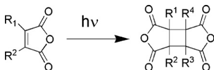
Scheme 17. Preparation of cis -cyclobutane-1,2,3,4-tetracarboxylic dianhydrides.
