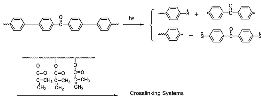
Scheme 55. The crosslinking reactions in negative photoresist [231].
