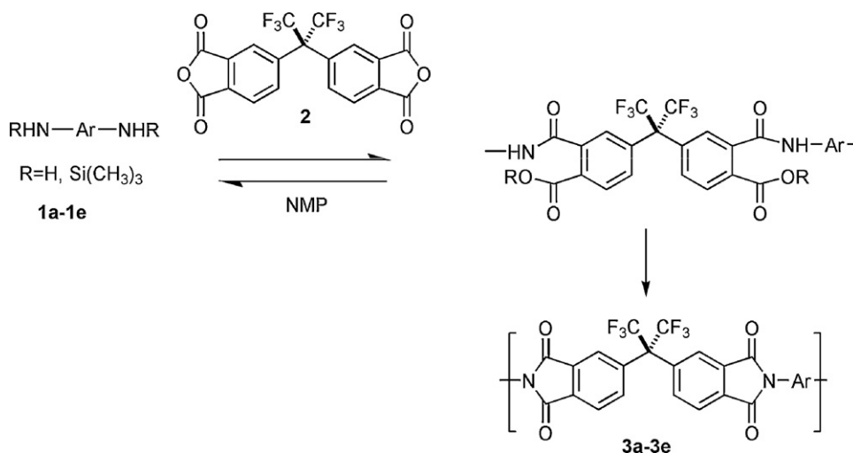
Scheme 48. Synthesis of polyimides from silylated diamines and dianhydrides.
