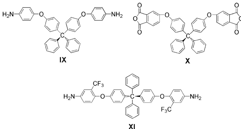
Scheme 2. Some structures of novel kink diamines and dianhydrides.
