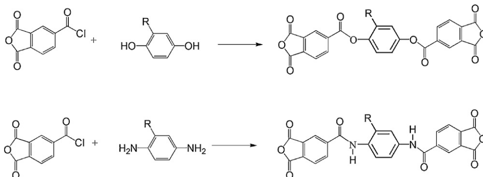
Scheme 42. Dianhydrides containing ester or amide groups [183].
