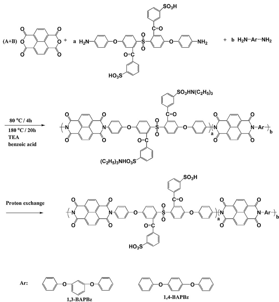
Scheme 68. Synthesis of BAPSBPS-based polyimides [168].
