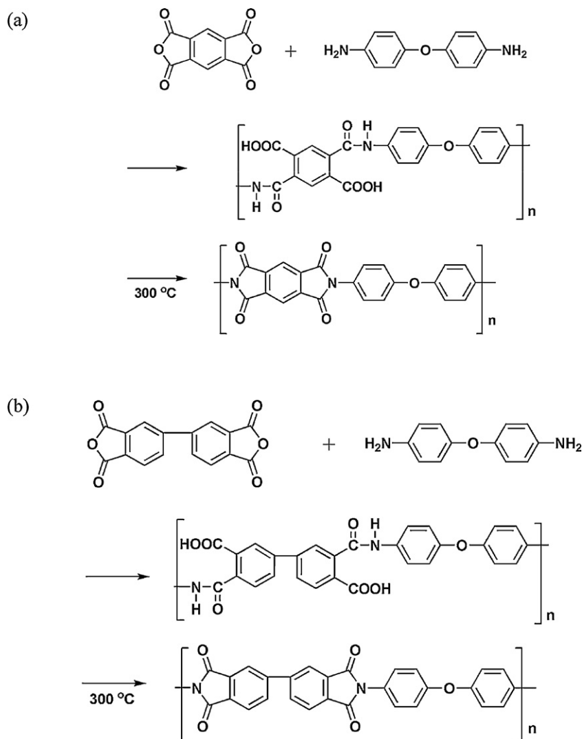
Scheme 50. (A) Synthesis of insoluble polyimide derived from 4,4'-oxydianiline and (B) synthesis of soluble polyimide derived from 4,4'-bipthalic anhydride.
