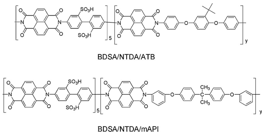
Scheme 67. Structures of BDSA/NTDA/mAPI and BDSA/NTDA/ATB [160].
