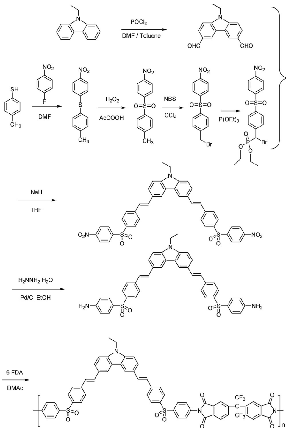
Scheme 30. Polyimides containing novel lambda-shaped two-dimensional carbazole chromophore.
