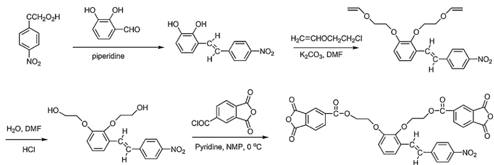
Scheme 38. Synthesis of Y-shaped NLO dianhydride [173].
