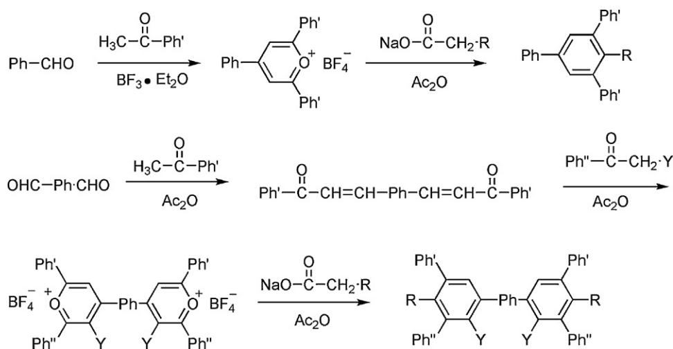
Scheme 10. Synthesis of rigid-rod noncoplanar and twisted diamines using pyrylium salts.
