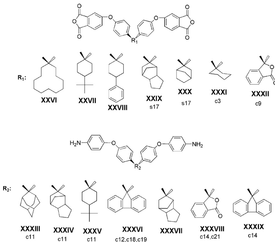
Scheme 7. Chemical structures of novel cardo monomers [23,30–34,36,78,79,448].
