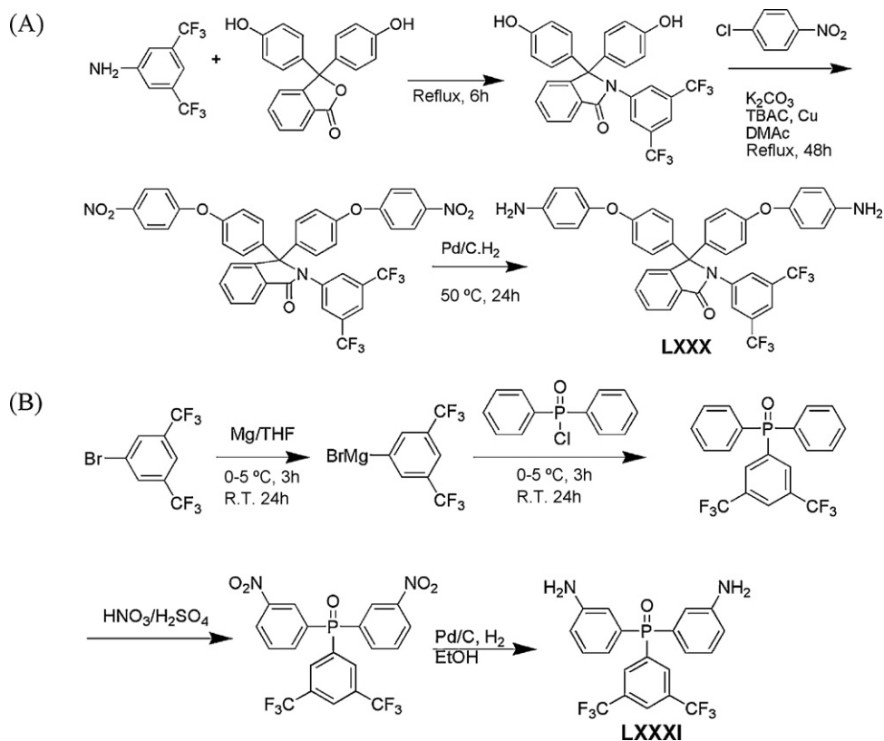
Scheme 23. Synthesis of 3,5-bis(trifluoromethyl)phenyl containing diamines [89,90].
