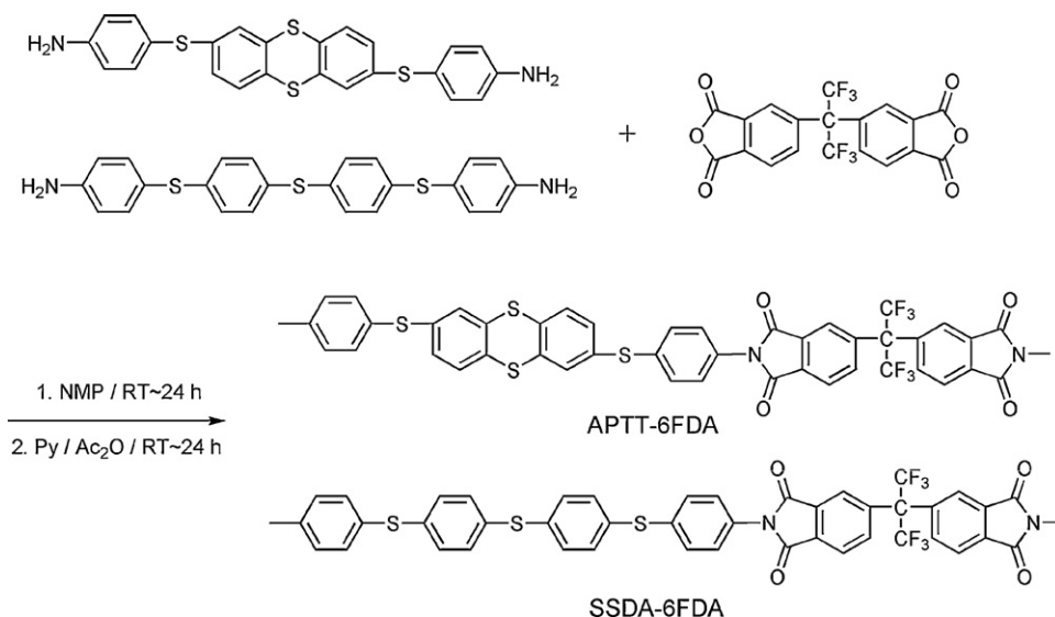
Scheme 82. Synthesis of two new sulfur-containing polyimides, APTT-6FDA and 3SDA-6FDA [430].
