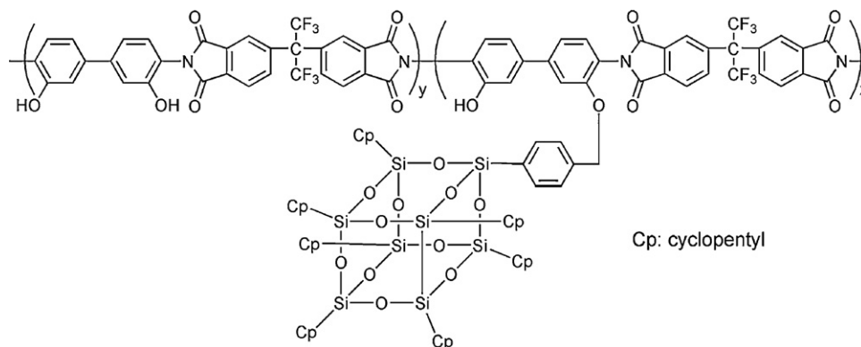
Scheme 26. Double-decker-shaped poly(silsesquioxane) (DDPSQ).
