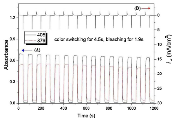
Fig. 4. (A) Potential step absorptometry and (B) current consumption of polyimide 1b (in \text{CH}_3\text{CN} with 0.1 M TBAP as the supporting electrolyte) by the application of a potential step 0–1.20 V.
