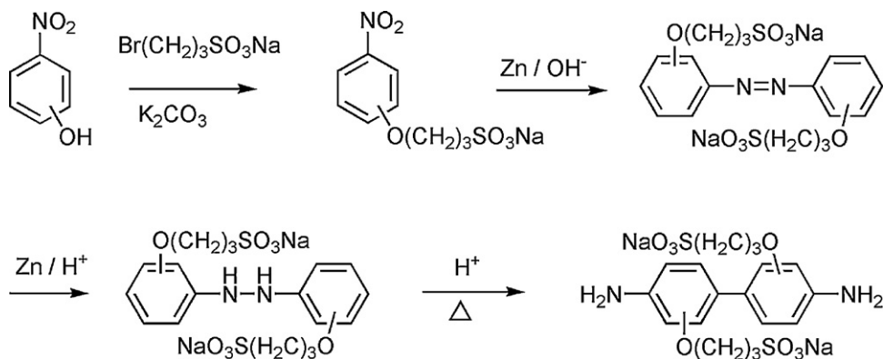
Scheme 36. Synthesis of sulfonated diamine isomers (BSPB) [166].
