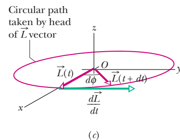
Figure 11-22 (a) A nonspinning gyroscope falls by rotating in an xz plane because of torque \vec{\tau} . (b) A rapidly spinning gyroscope, with angular momentum \vec{L} , precesses around the z axis. Its precessional motion is in the xy plane. (c) The change d\vec{L}/dt in angular momentum leads to a rotation of \vec{L} about O .
