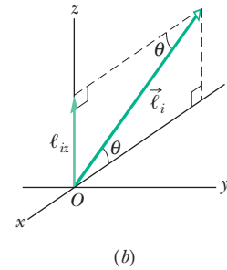
Figure 11-15 (a) A rigid body rotates about a z axis with angular speed \omega . A mass element of mass \Delta m_i within the body moves about the z axis in a circle with radius r_{\perp i} . The mass element has linear momentum \vec{p}_i , and it is located relative to the origin O by position vector \vec{r}_i . Here the mass element is shown when r_{\perp i} is parallel to the x axis. (b) The angular momentum vector \vec{\ell}_i , with respect to O , of the mass element in (a). The z component \ell_{iz} is also shown.
