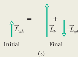
Figure 11-20 (a) A student holds a bicycle wheel rotating around a vertical axis. (b) The student inverts the wheel, setting himself into rotation. (c) The net angular momentum of the system must remain the same in spite of the inversion.
