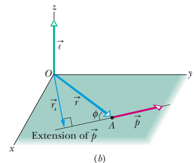
Figure 11-12 Defining angular momentum. A particle passing through point A has linear momentum \vec{p} ( = m\vec{v} ), with the vector \vec{p} lying in an xy plane. The particle has angular momentum \vec{\ell} ( = \vec{r} \times \vec{p} ) with respect to the origin O . By the right-hand rule, the angular momentum vector points in the positive direction of z . (a) The magnitude of \vec{\ell} is given by \ell = rp_{\perp} = rmv_{\perp} . (b) The magnitude of \vec{\ell} is also given by \ell = r_{\perp}p = r_{\perp}mv .
