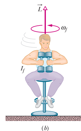
Figure 11-16 (a) The student has a relatively large rotational inertia about the rotation axis and a relatively small angular speed. (b) By decreasing his rotational inertia, the student automatically increases his angular speed. The angular momentum \vec{L} of the rotating system remains unchanged.
